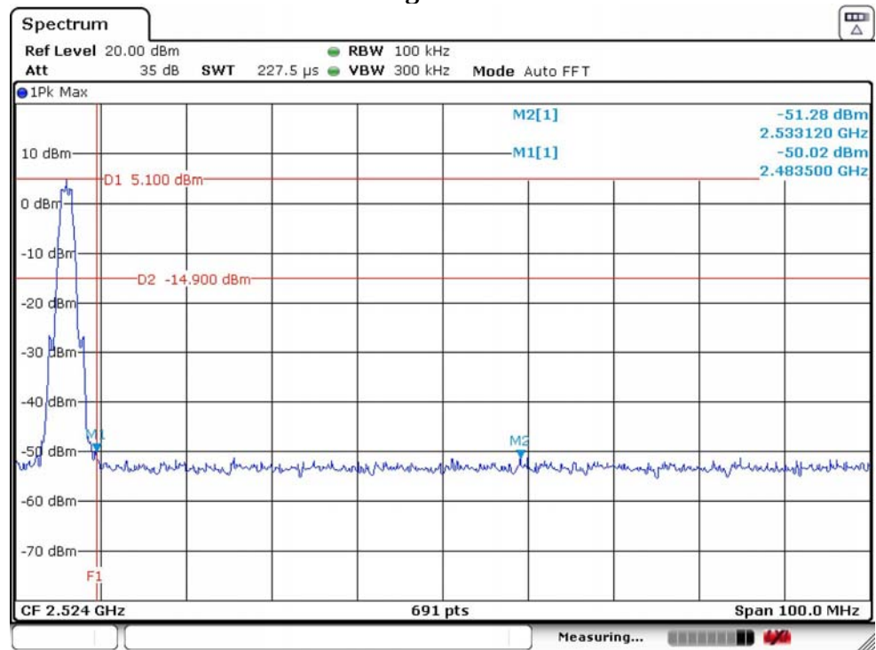
GFSK High Channel 2M
