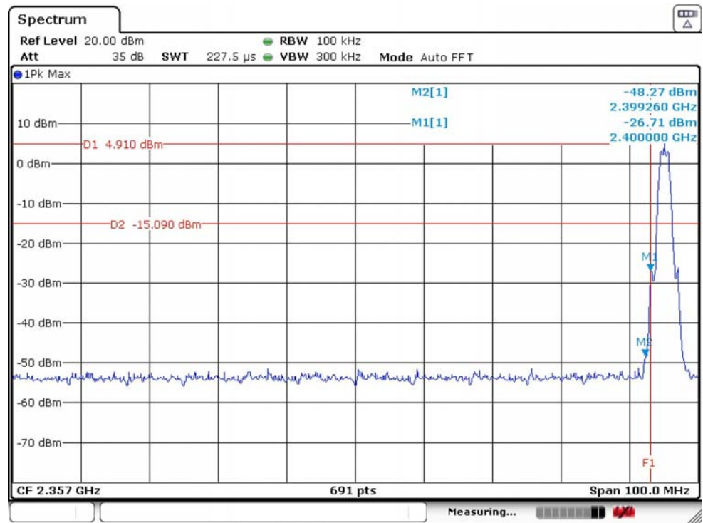
GFSK Low Channel 2M
