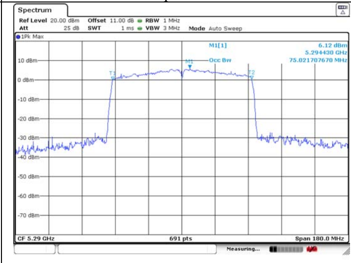
99% Occupied Bandwidth
