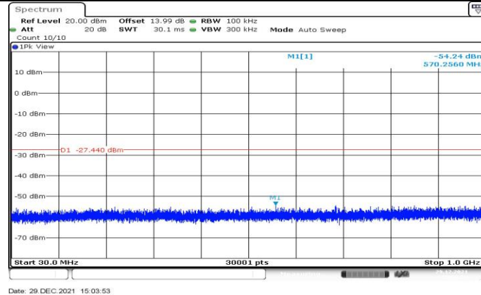
11N40MIMO Ant1 2452 30-1000
