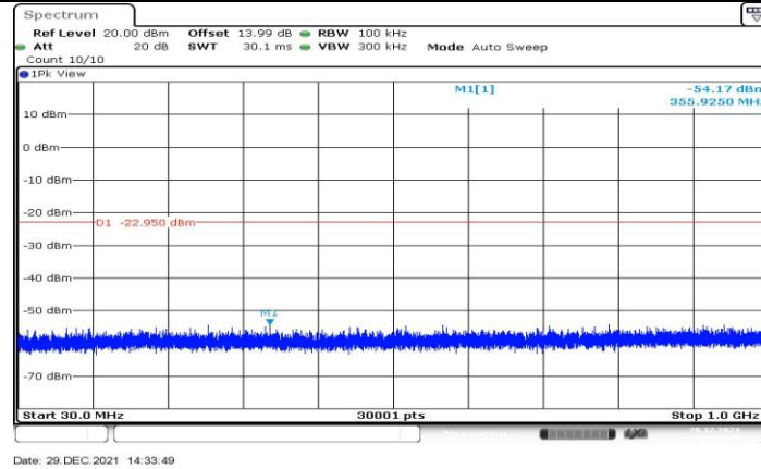
11B_Ant2_2437_30-1000
