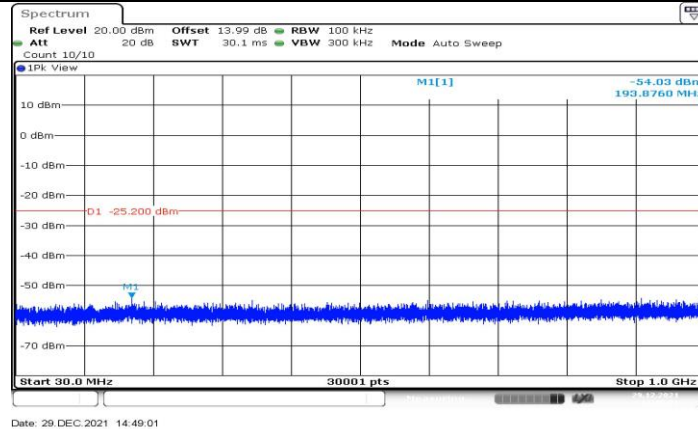
11N20MIMO Ant2 2437 30-1000
