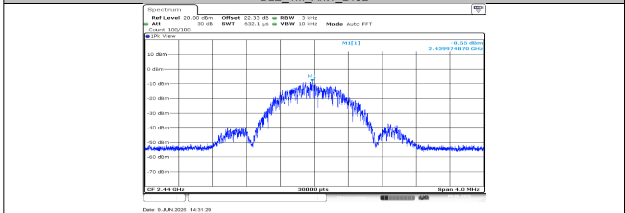
BLE_1M Ant1_2440
