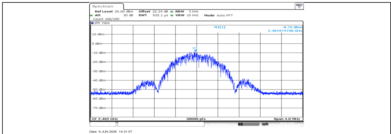
BLE_1M Ant1_2402
