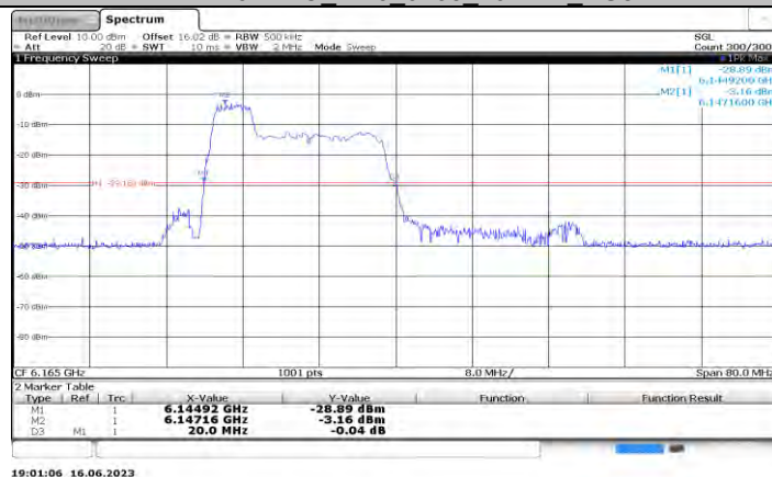
11AX40MIMO Ant0_6165_52Tone_RU37
