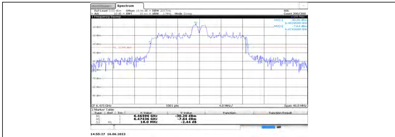
11AX20MIMO Ant0_6475_26Tone_RU4
