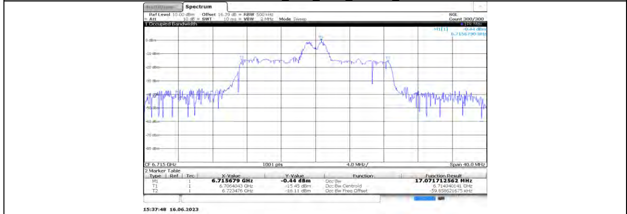
11AX20MIMO Ant0_6715_26Tone_RU4
