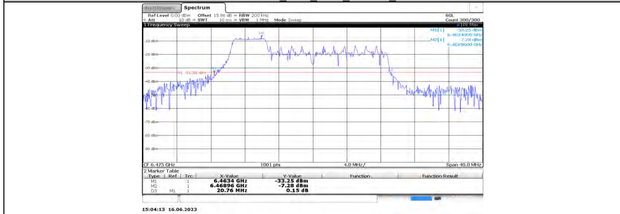
11AX20MIMO Ant0_6475_52Tone_RU37
