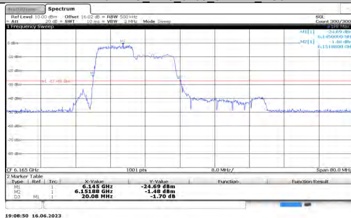
11AX40MIMO Ant0_6165_106Tone_RU53
