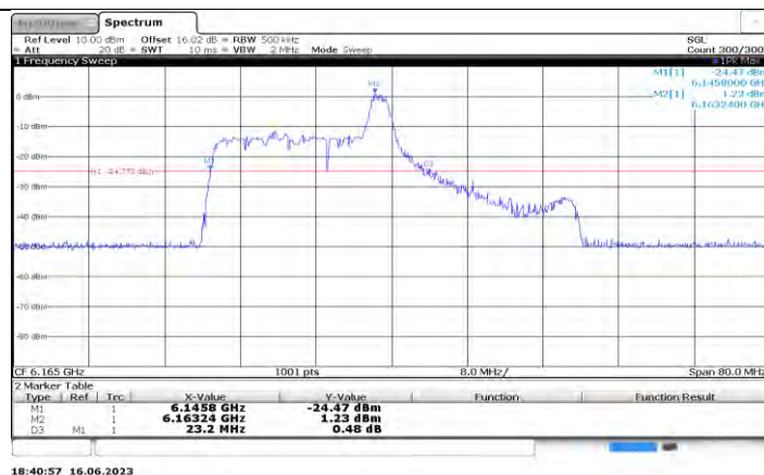
11AX40MIMO Ant0_6165_26Tone_RU8
