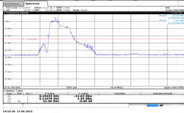
11AX80MIMO Ant0 6145_106Tone_RU53
