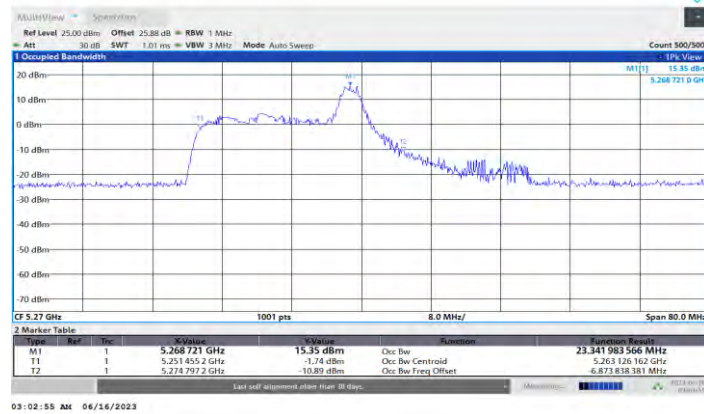
11AX40MIMO Ant1 5270 26Tone RU8
