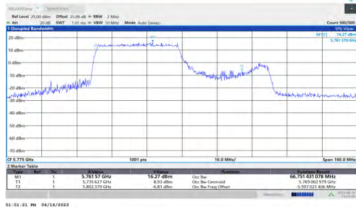
11AX80MIMO Ant1 5775 484Tone RU65
