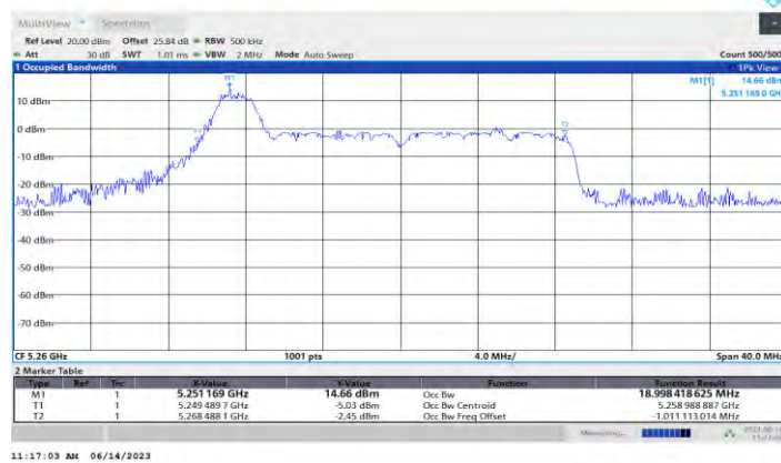
11AX20MIMO Ant1 5260 26Tone RU0
