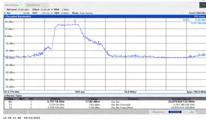
11AX80MIMO Ant1 5775 242Tone RU61
