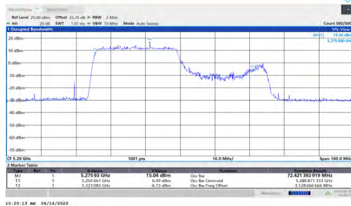
11AX80MIMO Ant0 5290 484Tone RU65
