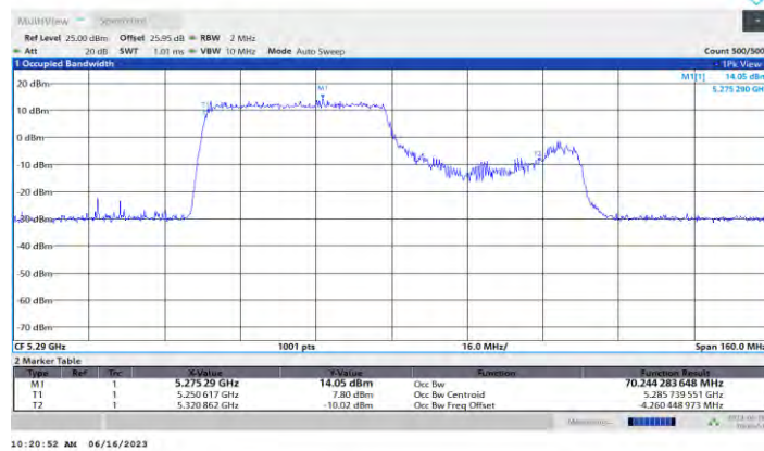
11AX80MIMO Ant1 5290 484Tone RU65
