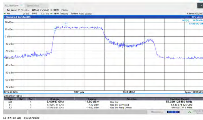
11AX80MIMO Ant1 5530 484Tone RU65
