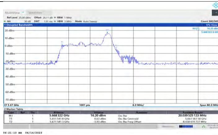
11AX40MIMO Ant1 5670 26Tone RU0
