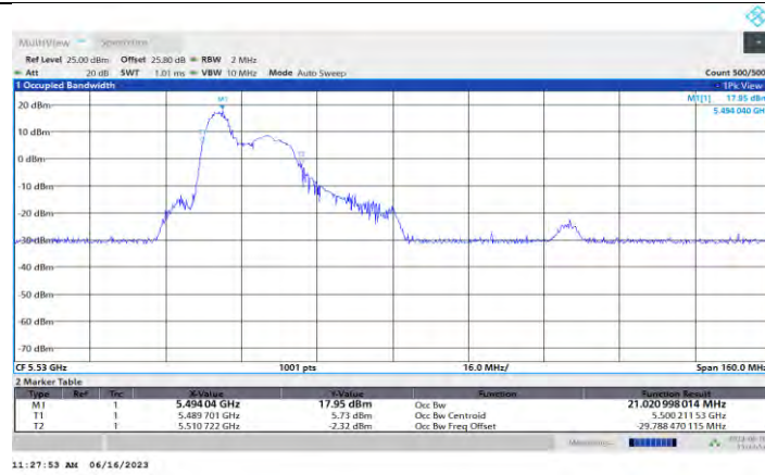
11AX80MIMO Ant0 5530 52Tone RU37
