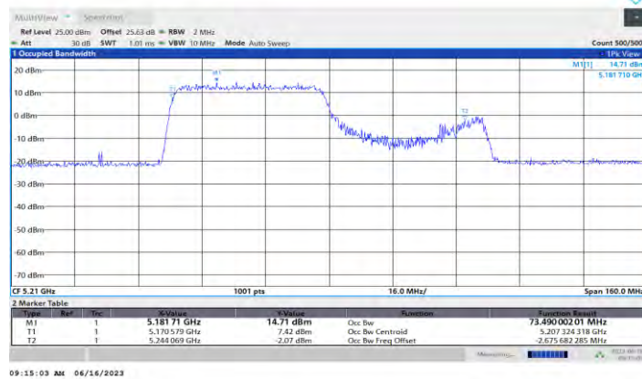
11AX80MIMO Ant0 5210 484Tone RU65
