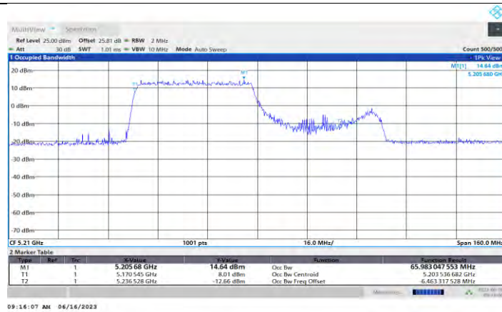
11AX80MIMO Ant1 5210 484Tone RU65
