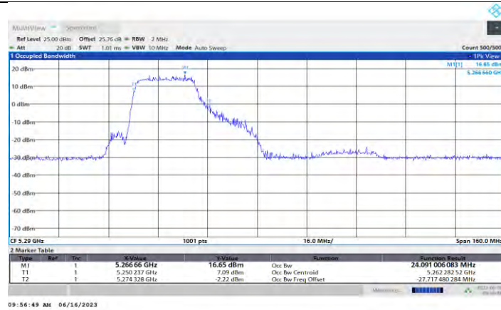
11AX80MIMO Ant0 5290 242Tone RU61
