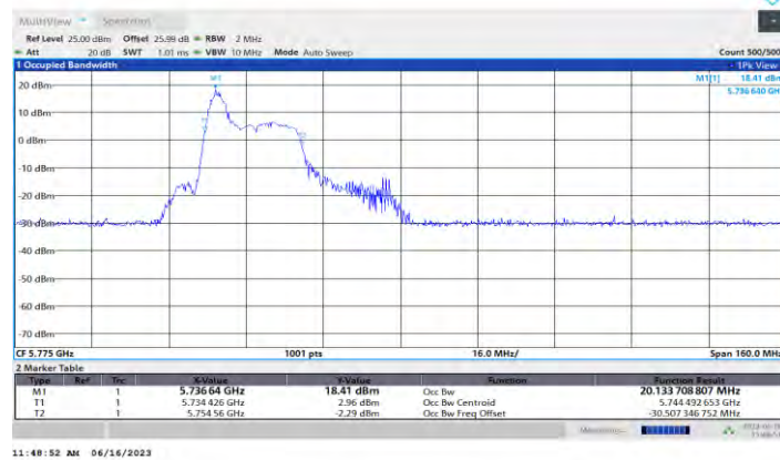
11AX80MIMO Ant1 5775 26Tone RU0
