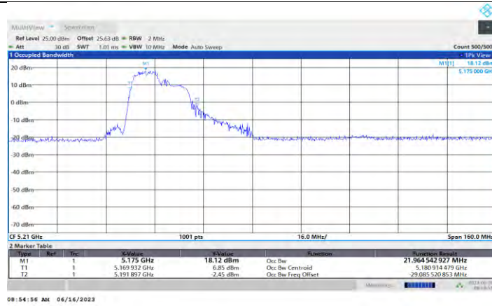
11AX80MIMO Ant0 5210 106Tone RU53
