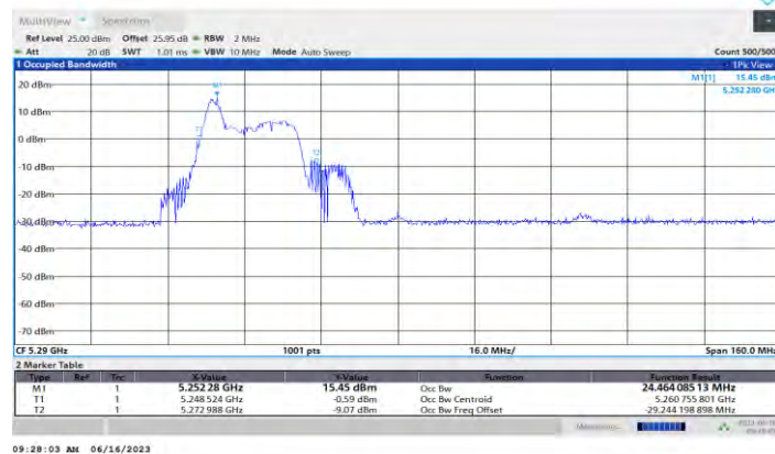
11AX80MIMO Ant1 5290 26Tone RU0
