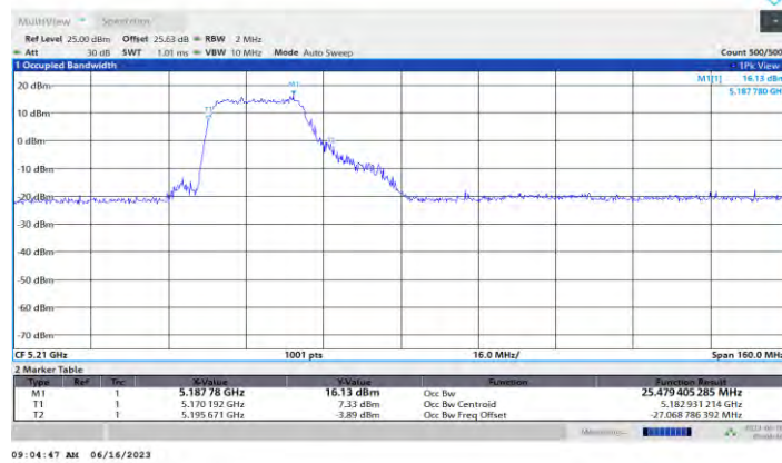
11AX80MIMO Ant0 5210 242Tone RU61
