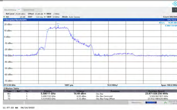
11AX80MIMO Ant1 5530 242Tone RU61
