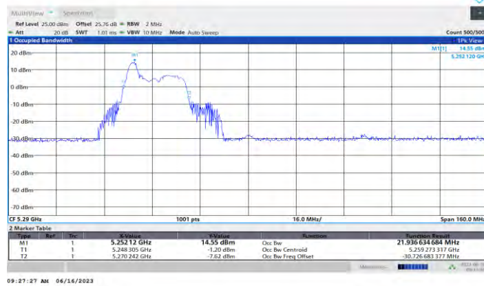
11AX80MIMO Ant0 5290 26Tone RU0
