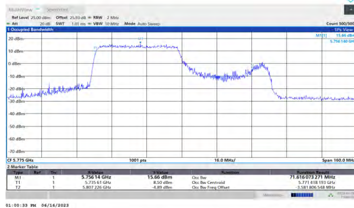
11AX80MIMO Ant0 5775 484Tone RU65
