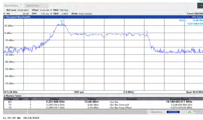
11AX20MIMO Ant0 5260 26Tone RU0
