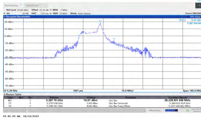
11AX80MIMO Ant0 5290 26Tone RU17
