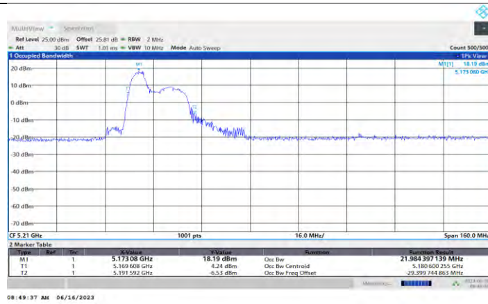
11AX80MIMO Ant1 5210 52Tone RU37
