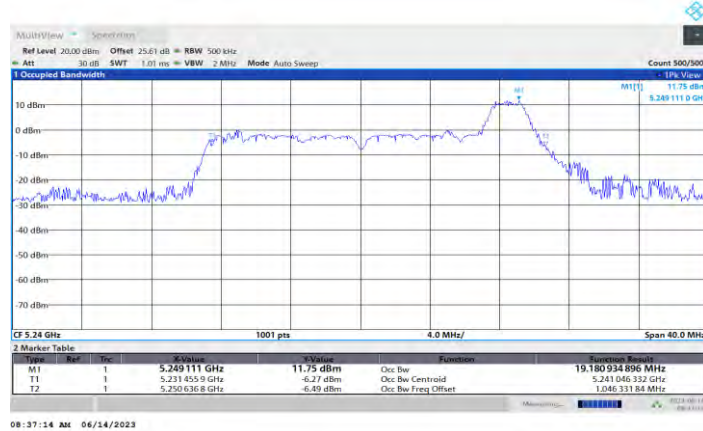
11AX20MIMO Ant0 5240 26Tone RU8
