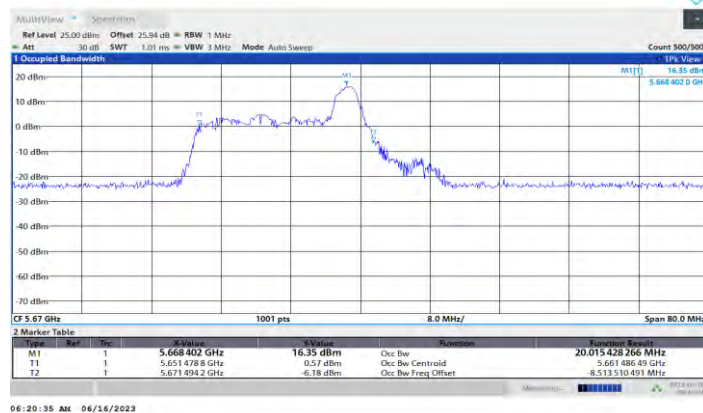
11AX40MIMO Ant0 5670 26Tone RU0
