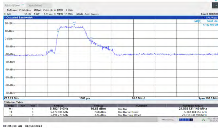
11AX80MIMO Ant1 5210 242Tone RU61
