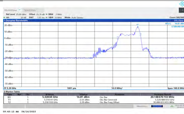
11AX80MIMO Ant0 5290 26Tone RU36
