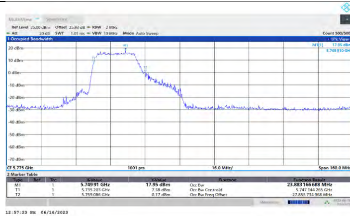
11AX80MIMO Ant0 5775 242Tone RU61
