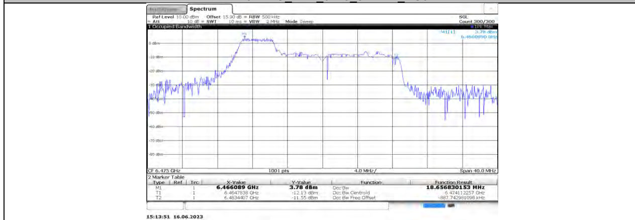
11AX20MIMO Ant1_6475_106Tone_RU53
