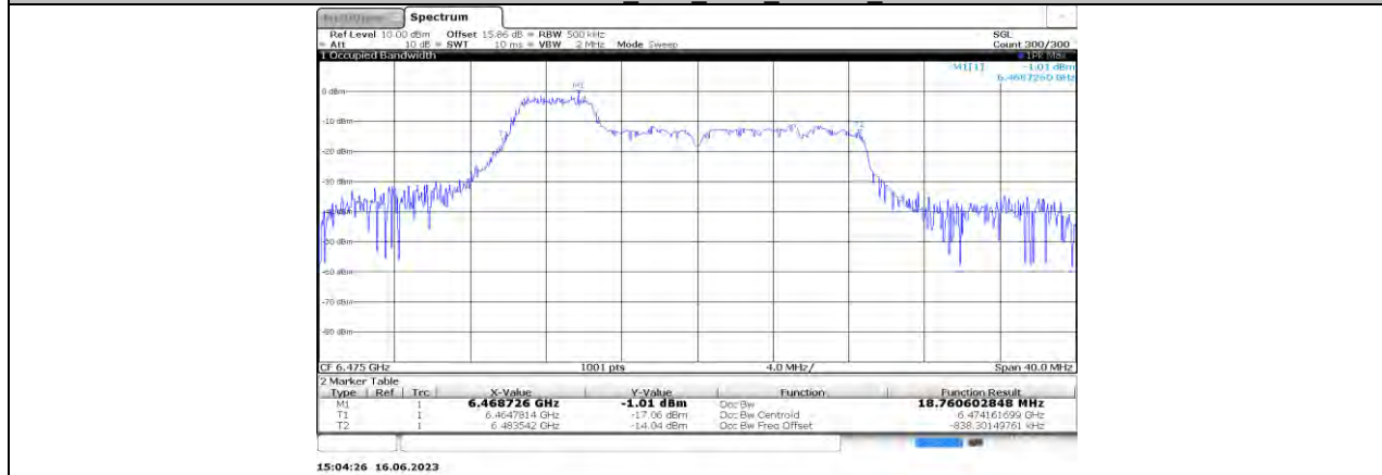
11AX20MIMO Ant0_6475_52Tone_RU37
