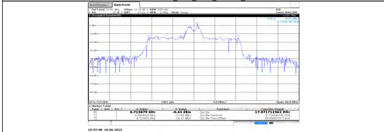
11AX20MIMO Ant0_6715_26Tone_RU4
