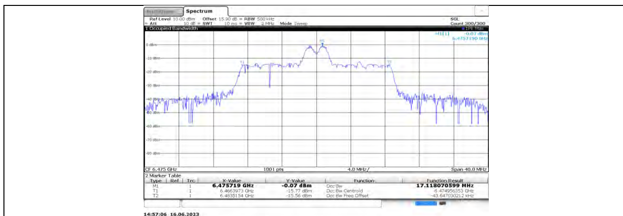
11AX20MIMO Ant1_6475_26Tone_RU4
