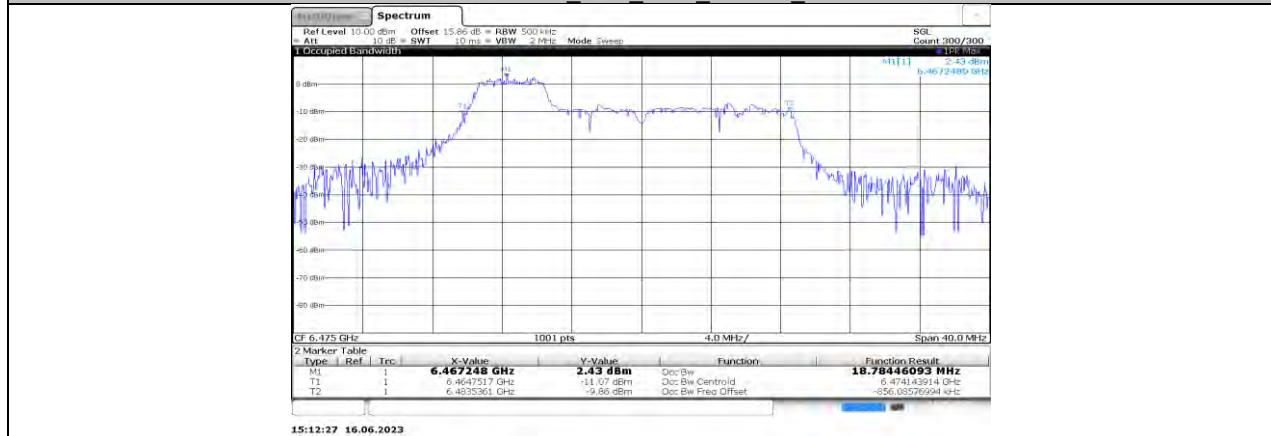
11AX20MIMO Ant0_6475_106Tone_RU53
