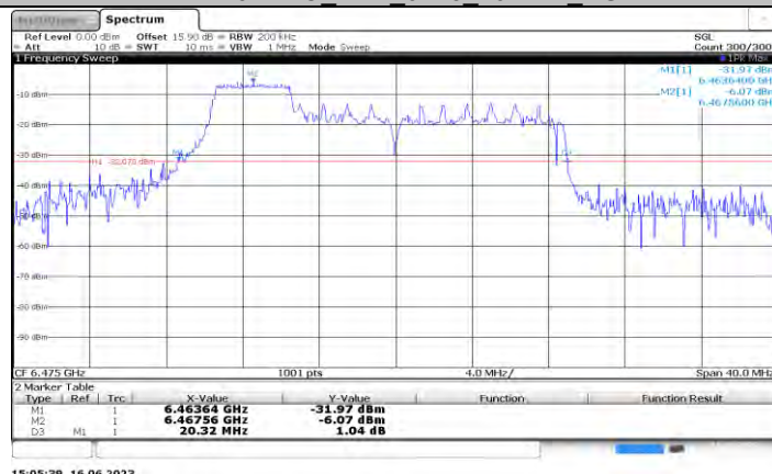
11AX20MIMO Ant1_6475_52Tone_RU37
