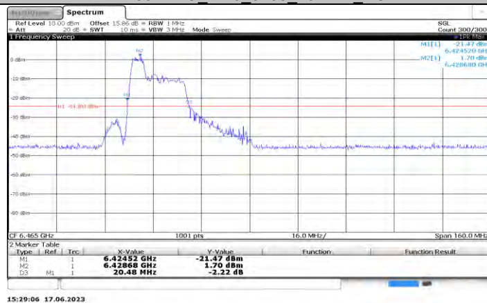
11AX80MIMO Ant0 6465 52Tone RU37
