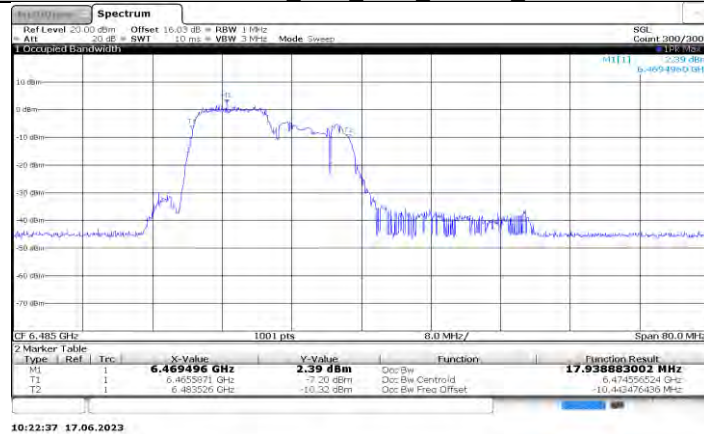
11AX40MIMO Ant0_6485_106Tone_RU53
