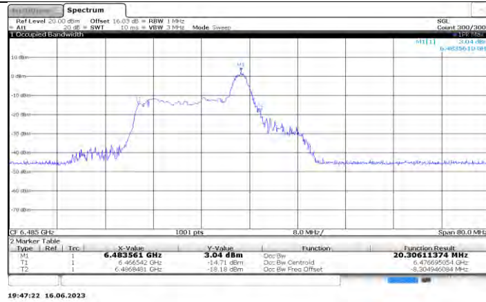
11AX40MIMO Ant0_6485_26Tone_RU8
