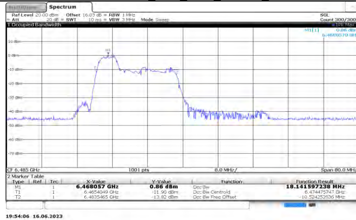
11AX40MIMO Ant0_6485_52Tone_RU37
