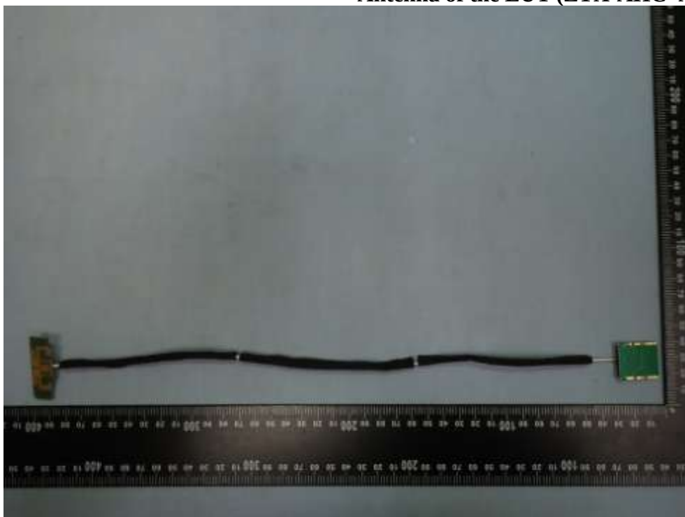
Figure 25 Antenna of the EUT (ZTX-AHC- Ant-2#-V02 )
