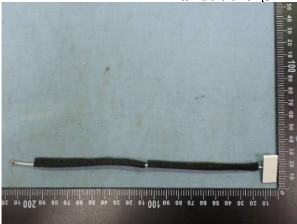
Figure 15 Antenna of the EUT (SH1-Ant-2#- V1.0 )
