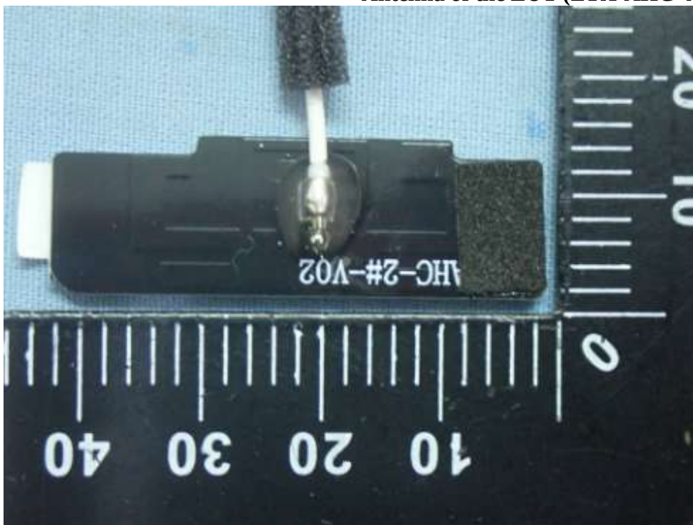
Figure 28 Antenna of the EUT (ZTX-AHC- Ant-2#-V02 )
