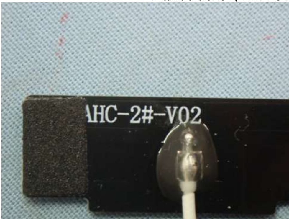
Figure 29 Antenna of the EUT (ZTX-AHC- Ant-2#-V02 )
