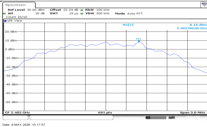
BLE_2M_Ant2_2402_0~Reference
