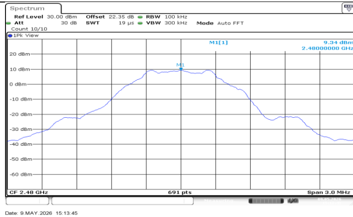
BLE_1M_Ant2_2480_0~Reference
