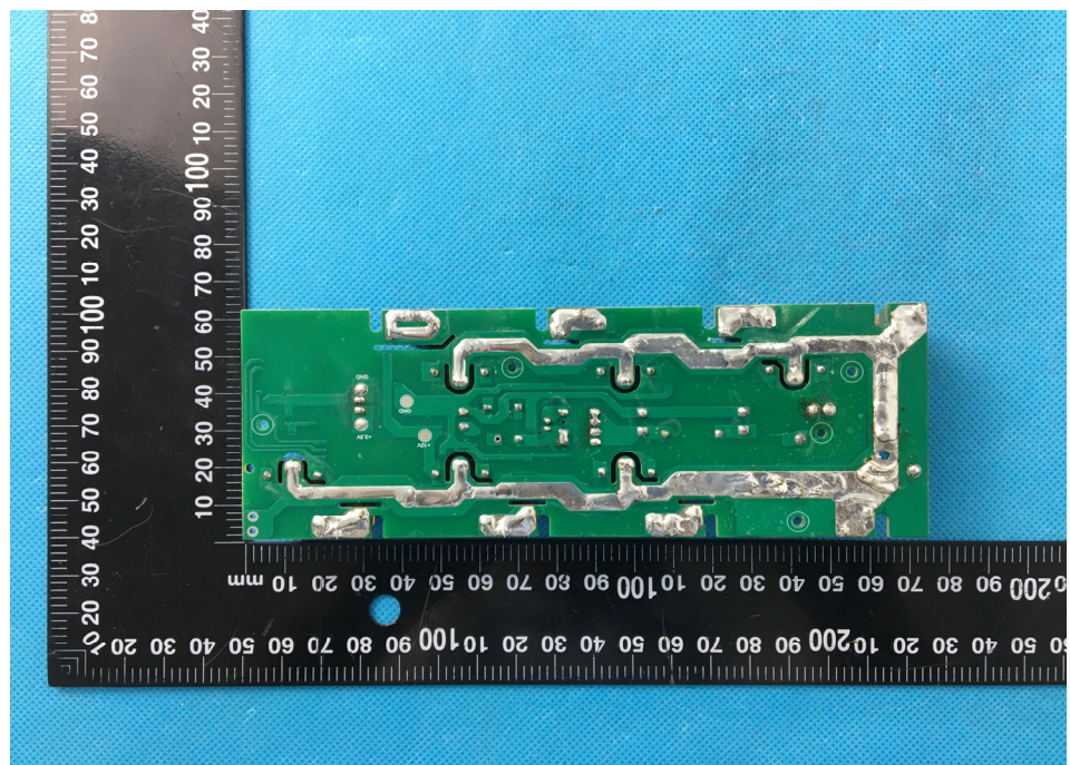
Solder Board-Component View 4
