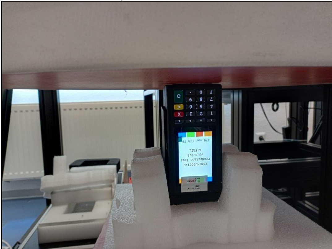
Photo 13: Test position - Bottom side with 0mm distance
