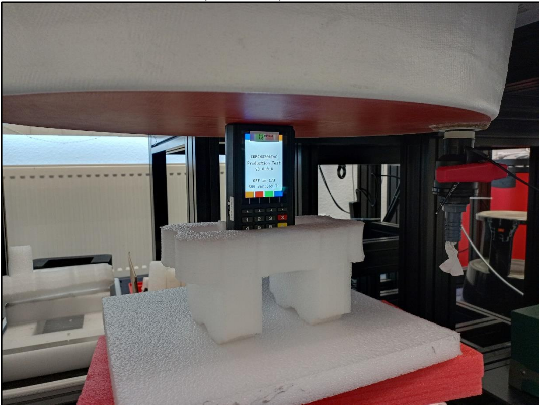
Photo 10: Test position - Top side with 0mm distance
