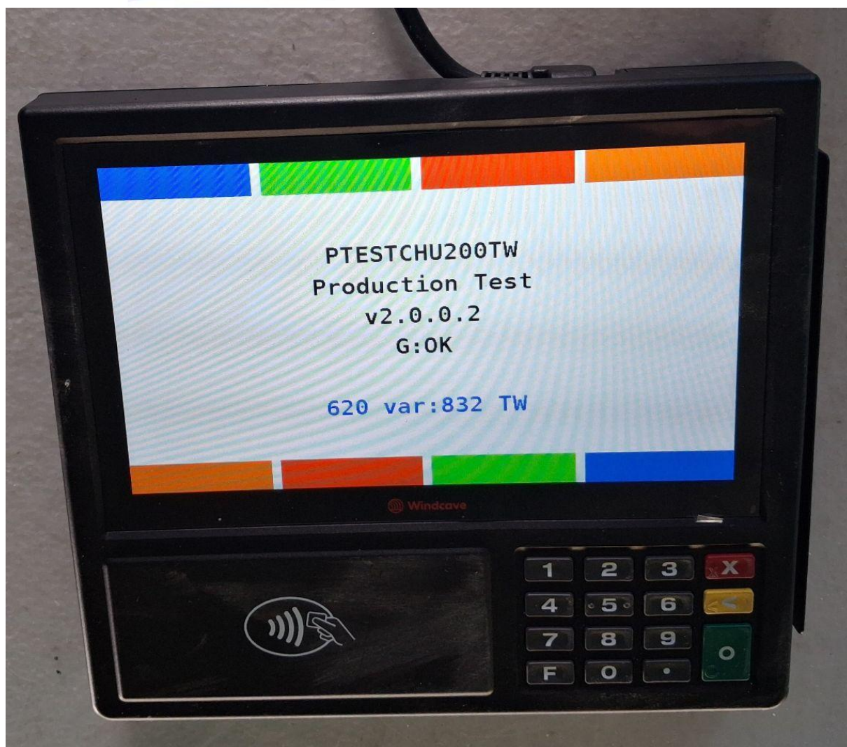
Device under test – Front Face
