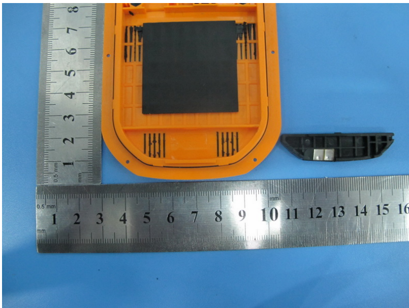
Photo 17 Appearance of Antenna
