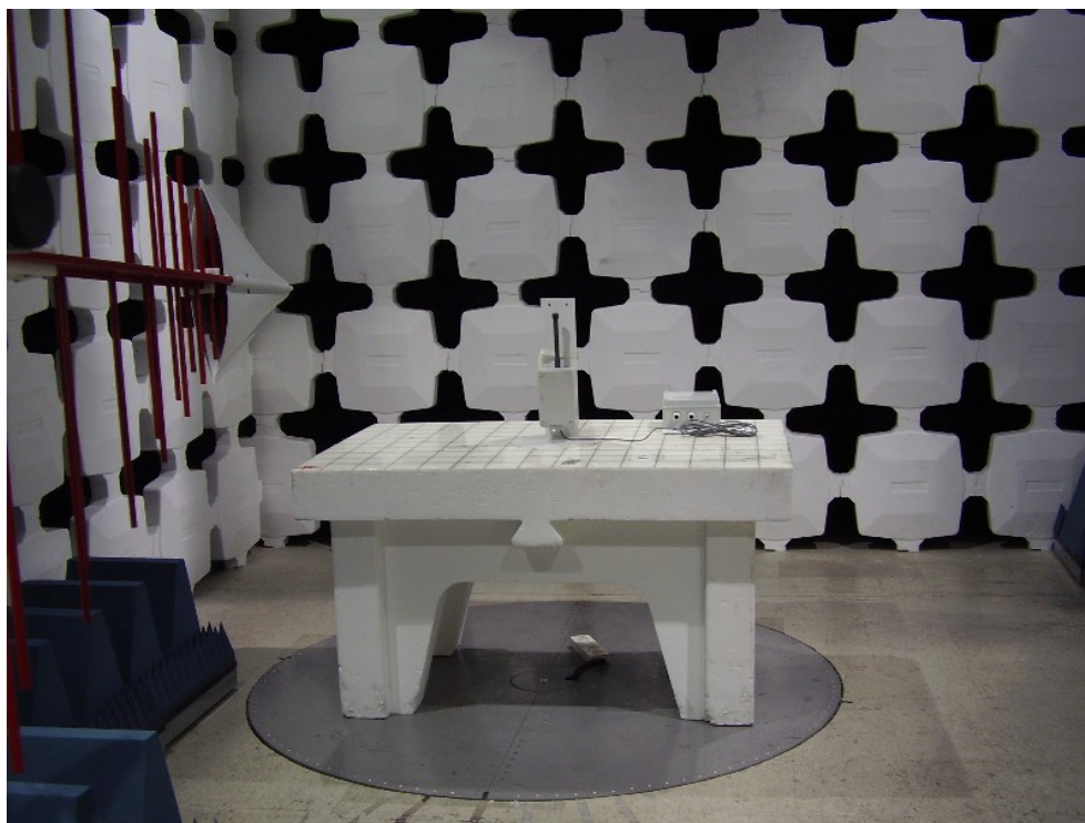
Photo 2. Radiated emissions test.
