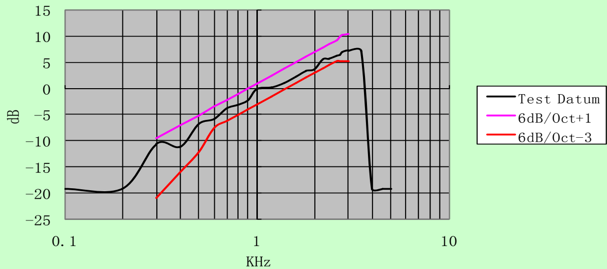
Audio Frequency Response for 12.5KHz
