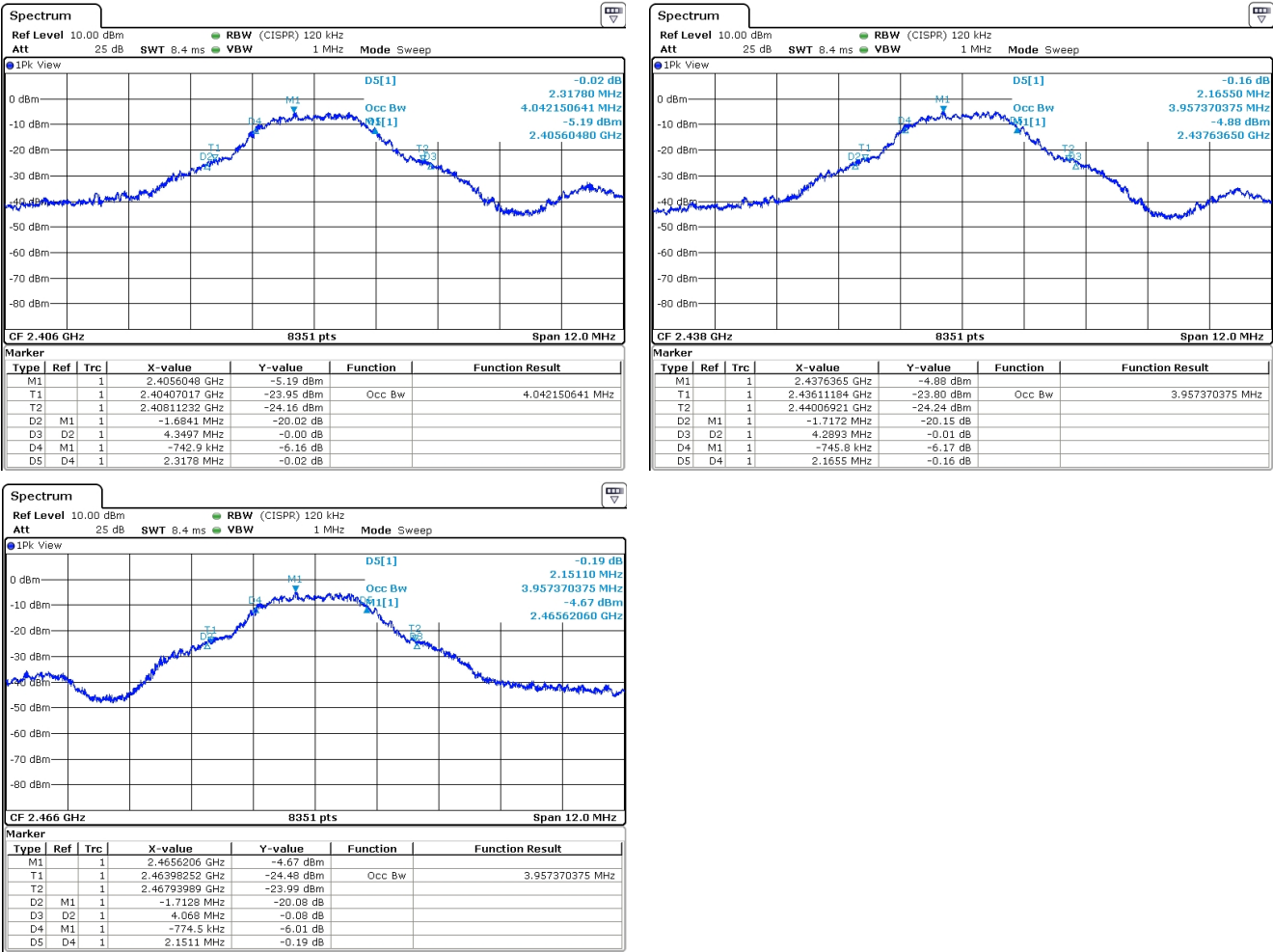
Figure 8: Intentional Emission Bandwidth.
