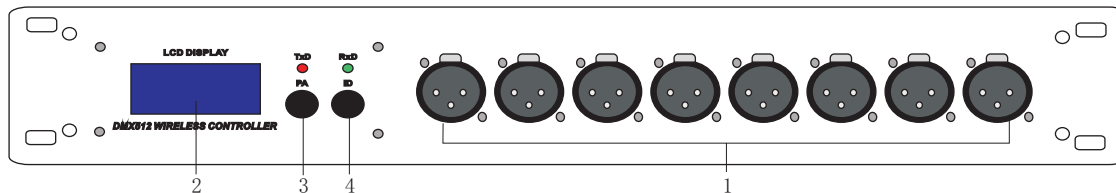
Front board
