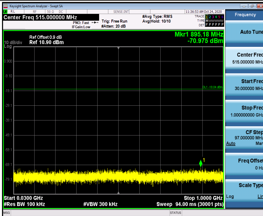
2DH5_Ant1_2441_30~1000
