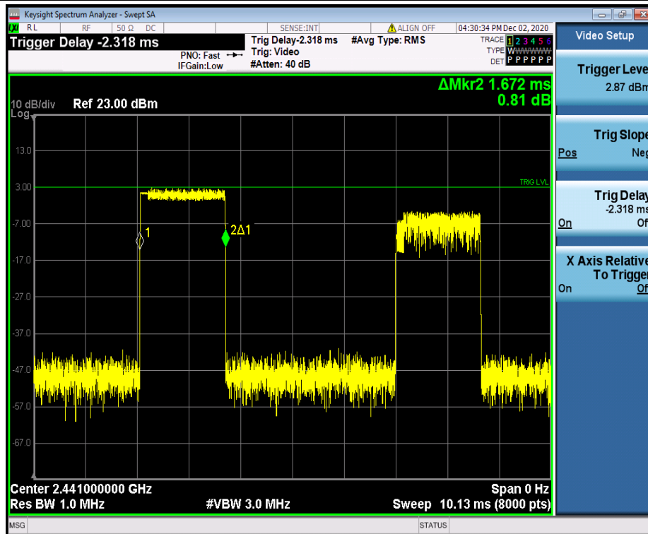
3DH3_Ant1_Hop_2441
