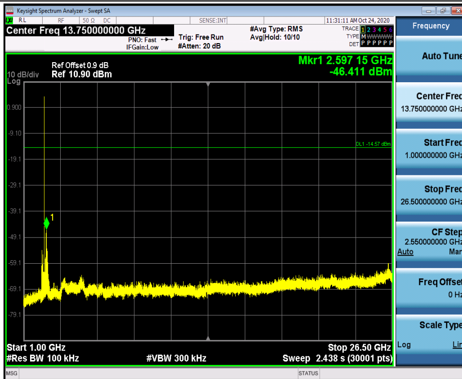
DH5_Ant1_2441_1000~26500
