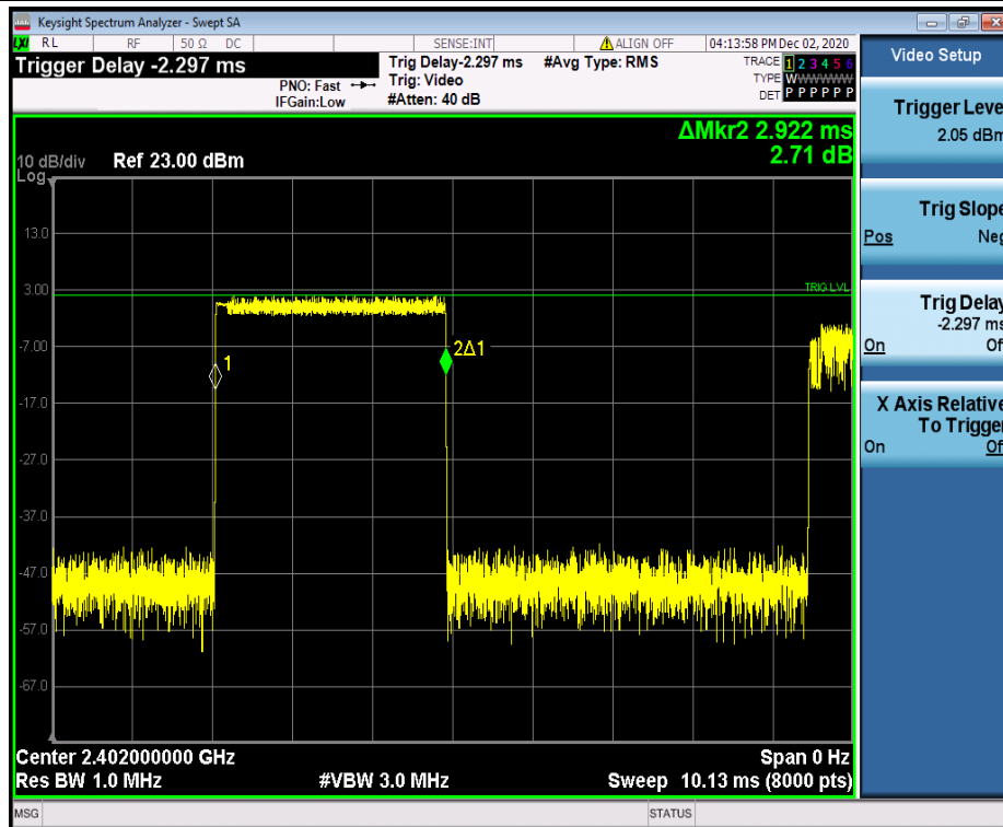
3DH5_Ant1_Hop_2402
