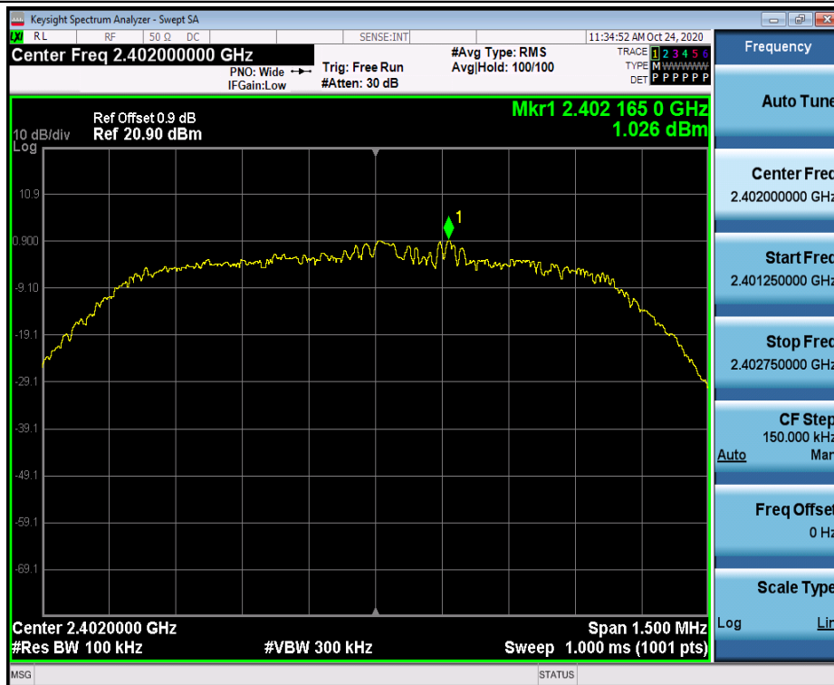
2DH5_Ant1_2402_0~Reference
