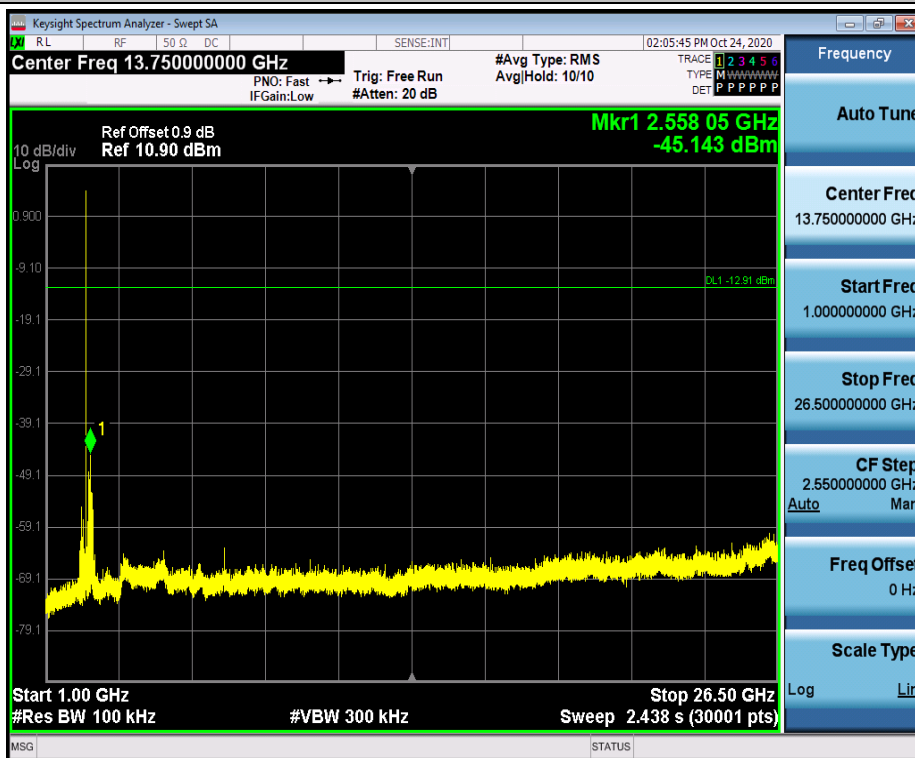
BLE_1M_Ant1_2440_0~Reference
