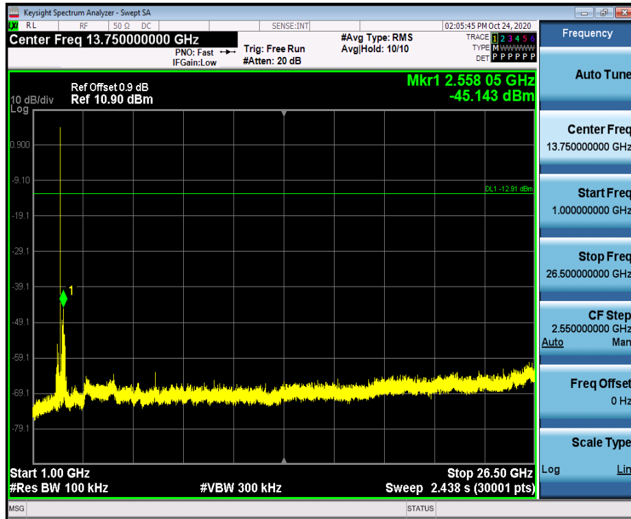
BLE_1M_Ant1_2440_0~Reference
