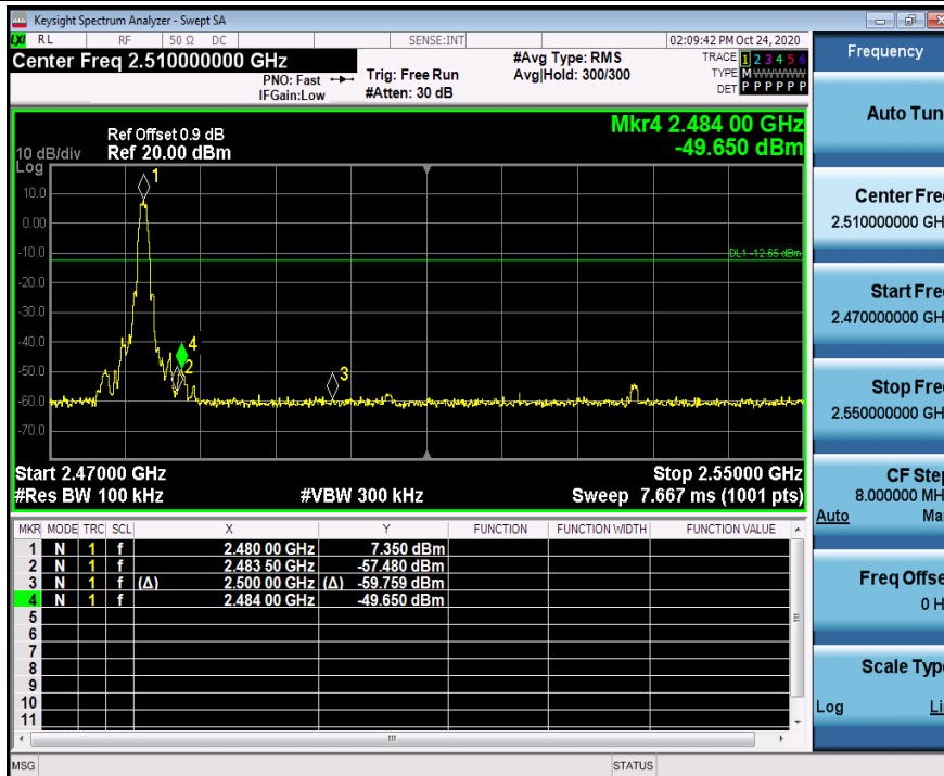
BLE_1M_Ant1_High_2480
