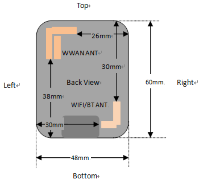
Fig.14.1 EUT Antenna Locations
