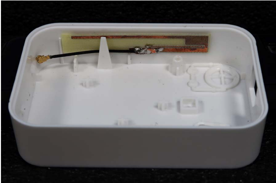
Antenna PCB in Case
