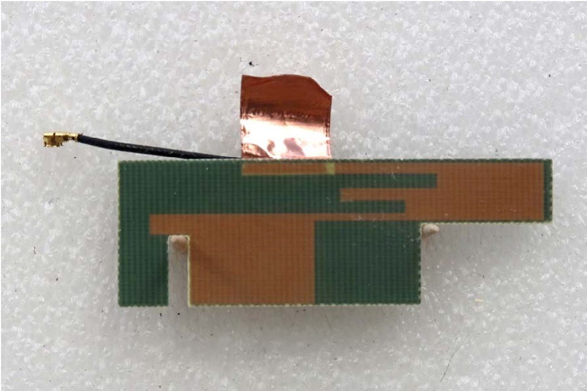
Antenna Front
