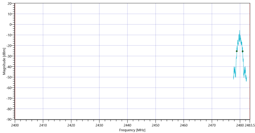
Plot_FCC Part 15.247 Bandwidth 99PCT-20dB ~ BT LE 2 Msps 24032021_095752.png
