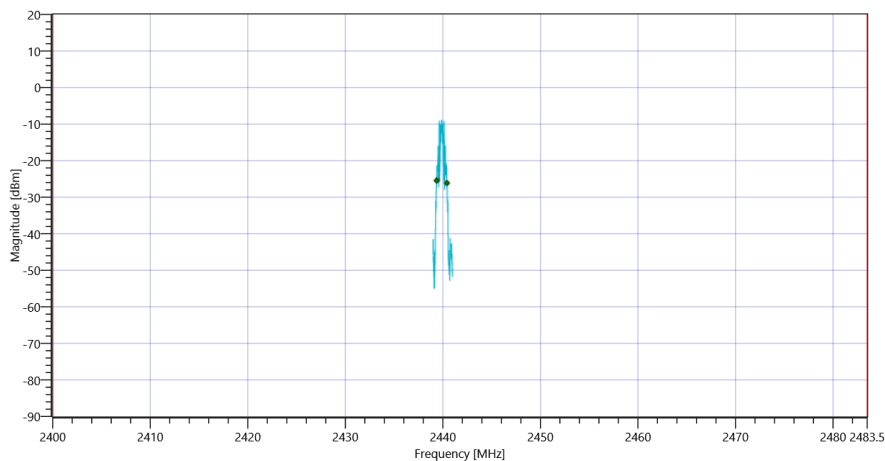
Plot_FCC Part 15.247 Bandwidth 99PCT-20dB ~ BT LE coded S8_24032021_102513.png
