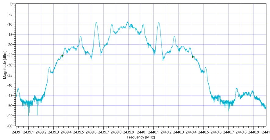
Plot_FCC Part 15.247 Bandwidth 99PCT-20dB ~ BT LE coded S8 99PCT_24032021_102506.png
