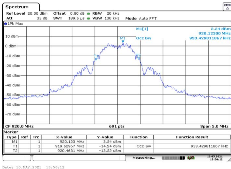
Plot 4: High Channel, 99%OBW
