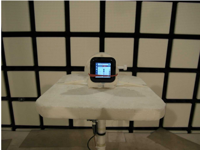
Photo 1 RSE > 1GHz
