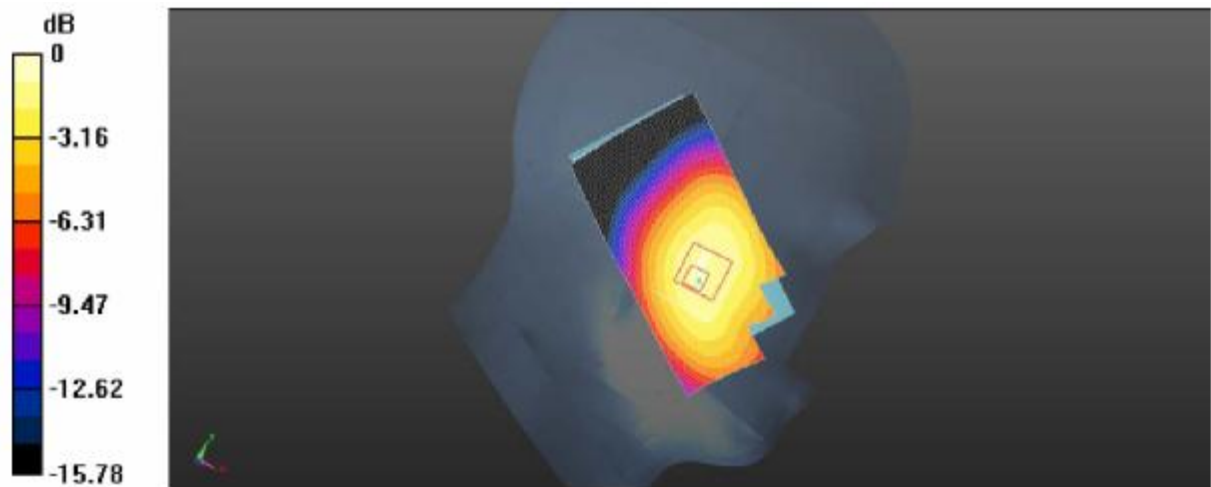
Plot 1: Left Head Tilt (GSM850 Middle Channel)
