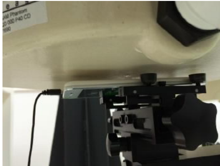
10mm Body-worn Rear(with Headset) Setup Photo
