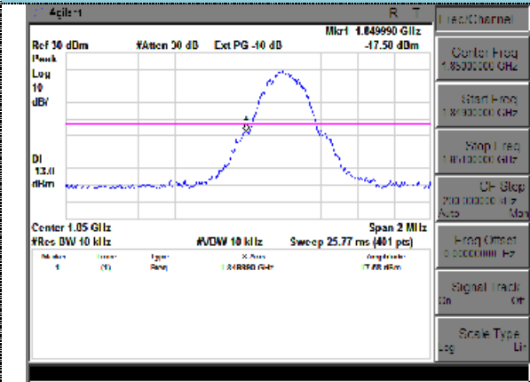
Channel 512
