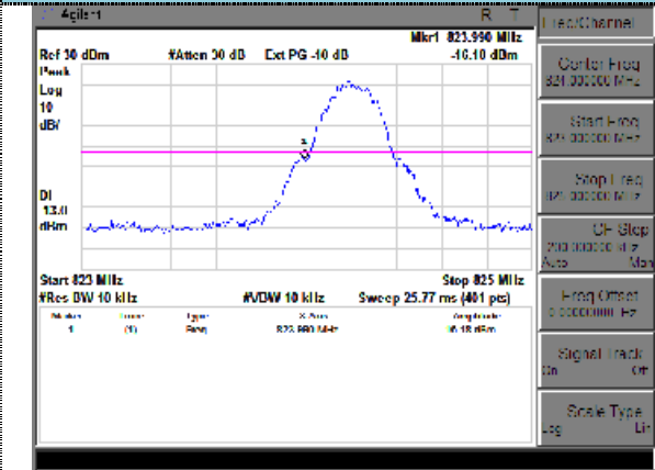
Channel 128
