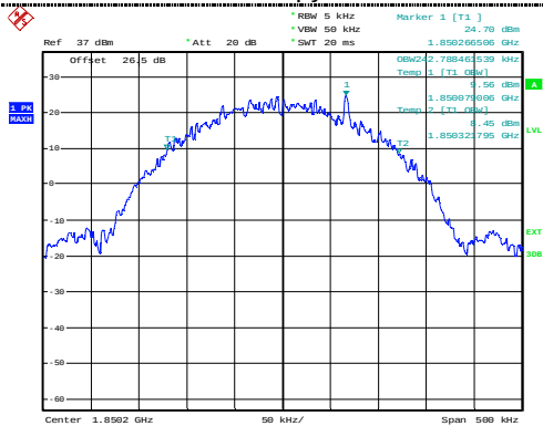
99% Occupty bandwidth
