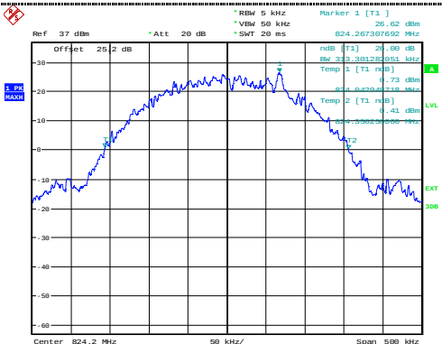
-26dB bandwidth
