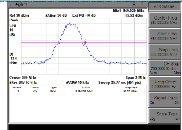
Channel 251
