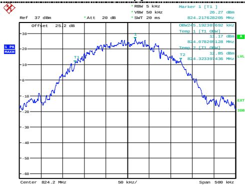
99% Occupy bandwidth
