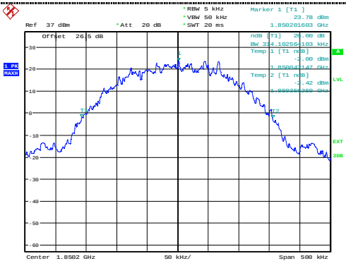
-26dB bandwidth
