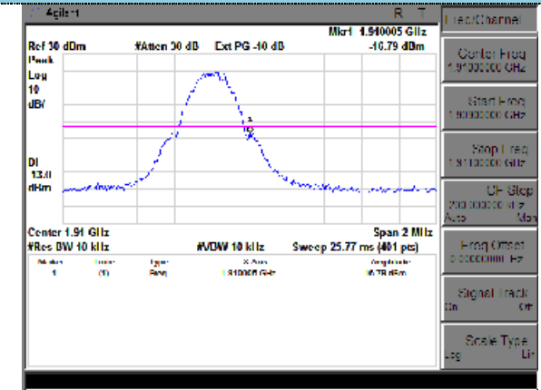
Channel 810
