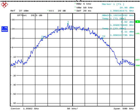
99% Occupancy bandwidth
