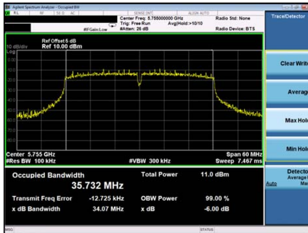
(802.11 AC40) 6dB Bandwidth plot on channel 151
