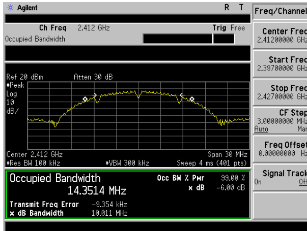
(802.11b) channel 1
