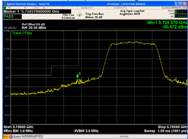
802.11n(HT20) U-NII-3 Band edge-left side
