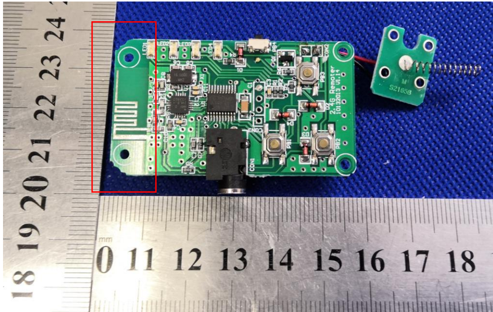
PCB view
