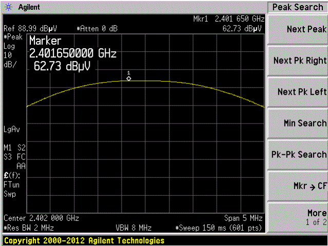
Vertical Polarity
