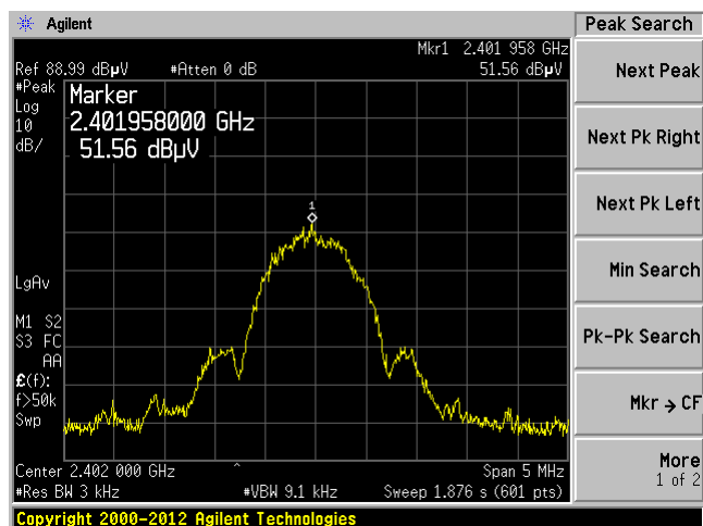
Horizontal Polarity
