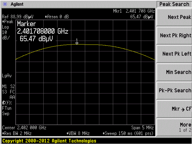
Horizontal Polarity
