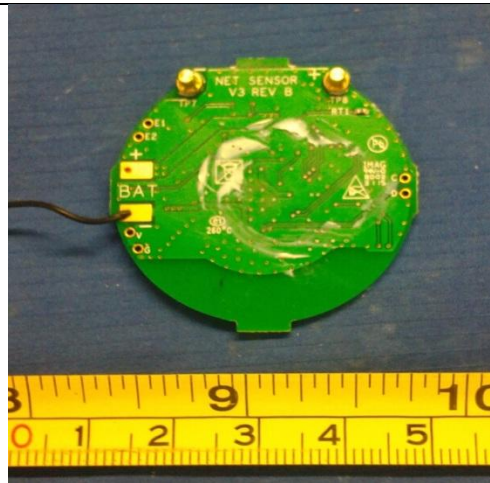
PCBA Top View
