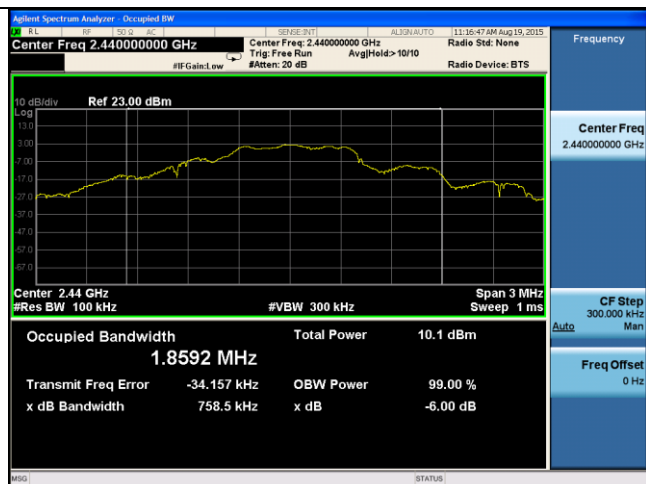
99% BW -Bluetooth LE 2440MHz
