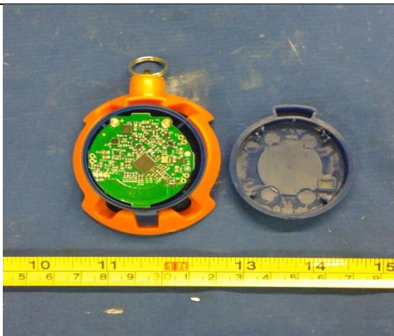
EUT Cover Off View 1
