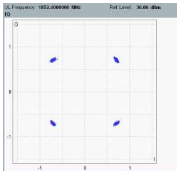
QPSK modulation
