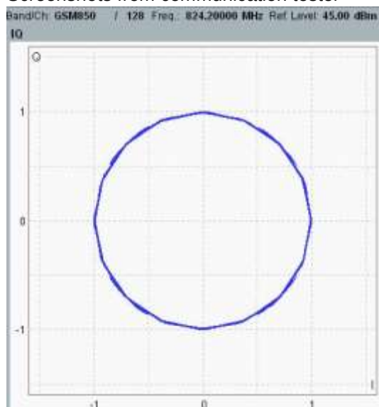
GMSK modulation
