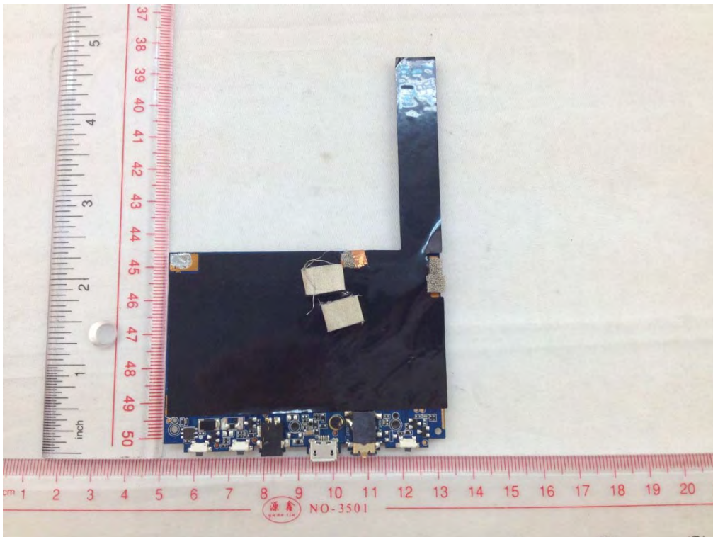
MAIN BOARD DOWN VIEW 1
