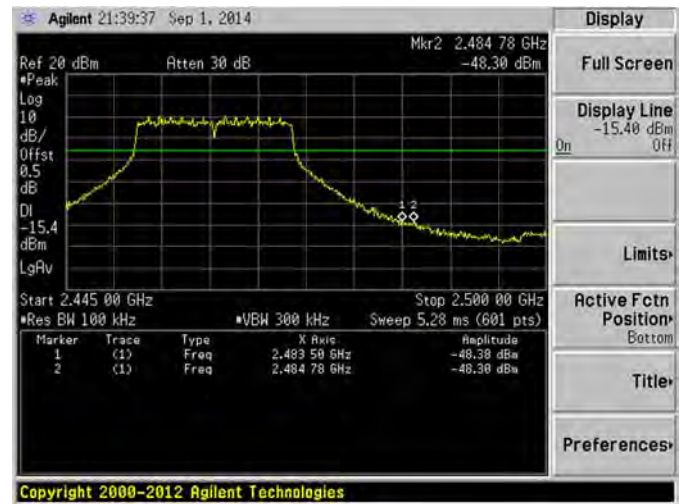
802.11n-20MHz HIGH CHANNEL, Band Edge
