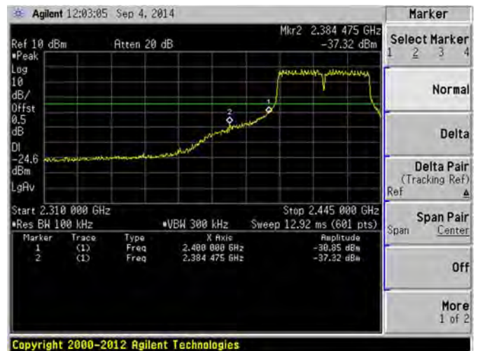
802.11n-40MHz LOW CHANNEL, Band Edge
