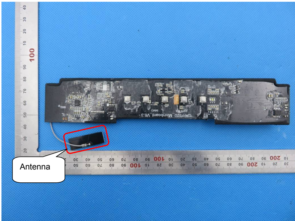
INTERNAL VIEW OF EUT-2 (Black)
