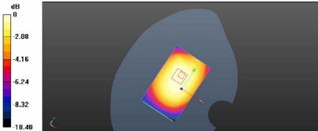
Plot 8: Body- worn Rear side (WLAN802.11b Middle Channel)
