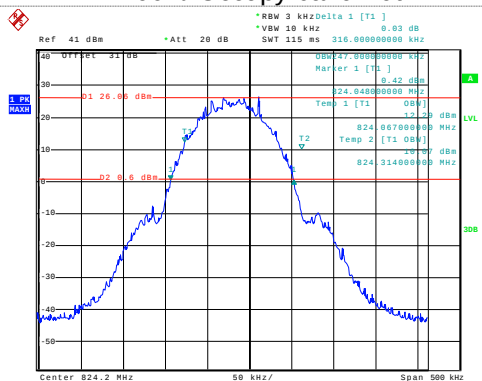
99% Occupy bandwidth
