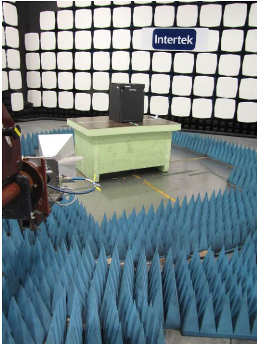
Radiated emissions measurements above 1 GHz
