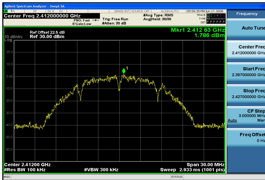
11B-Ant1-2412-0~Reference-PASS
