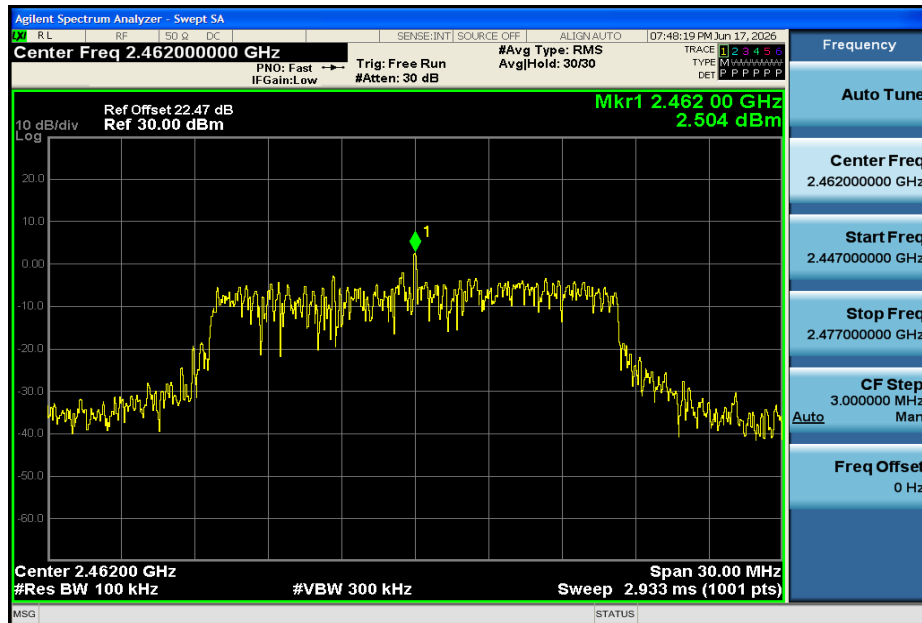
11G-Ant1-2462-0~Reference-PASS
