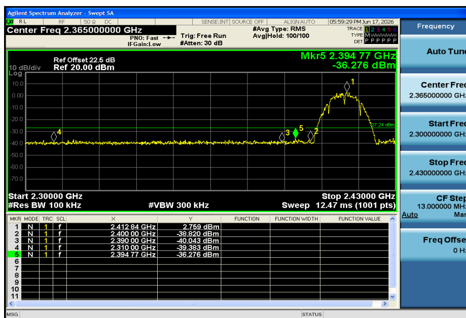
11B-Ant1-2412-PASS
