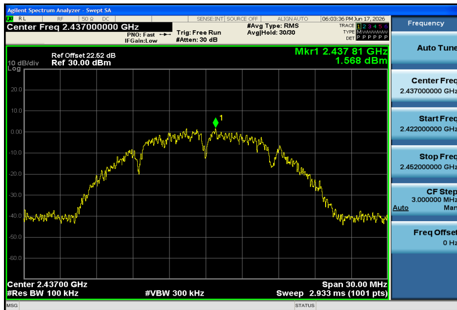
11B-Ant1-2437-0~Reference-PASS
