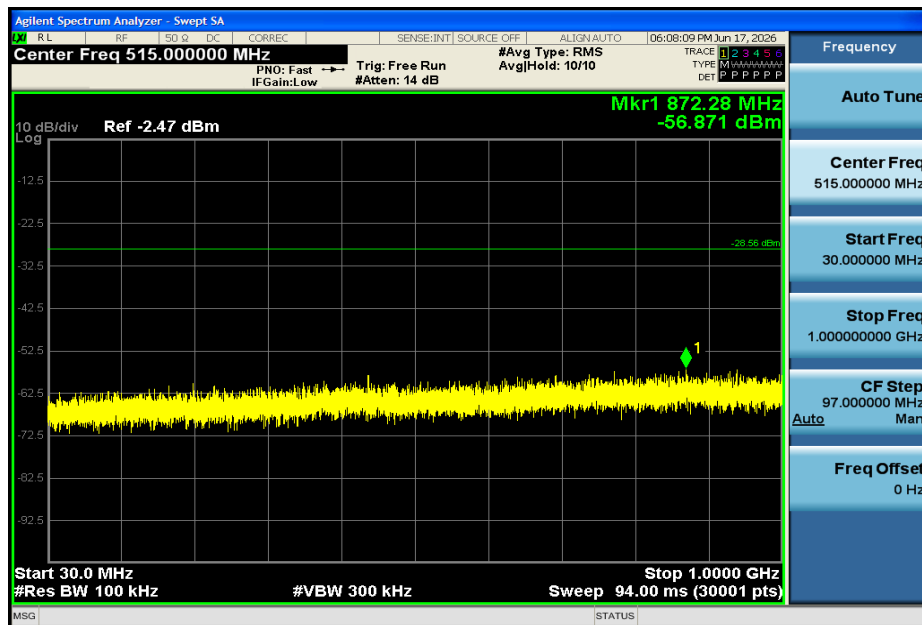
11B-Ant1-2462-30~1000-PASS
