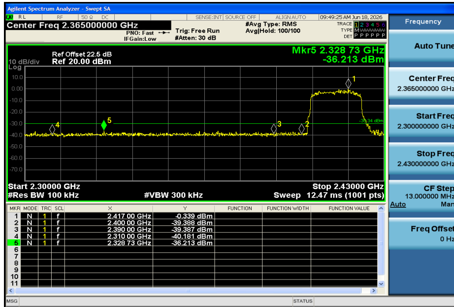
11AX20SISO-Ant1-2412-PASS
