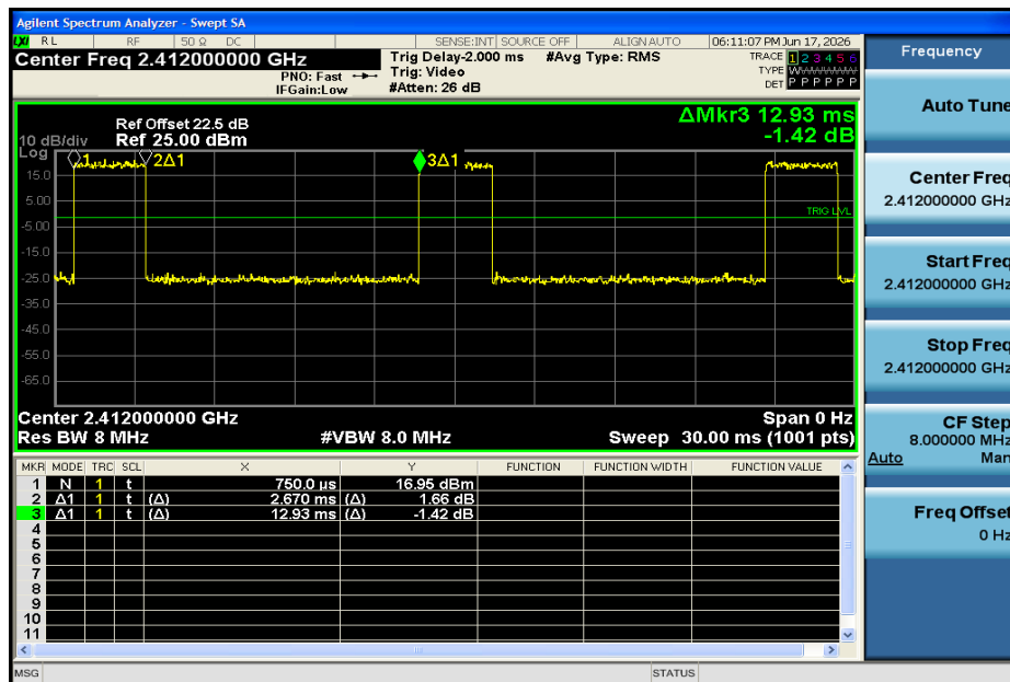
NTNV-11G-2412
