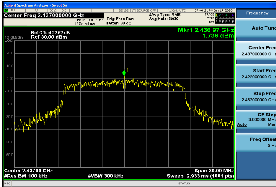
11G-Ant1-2437-0~Reference-PASS
