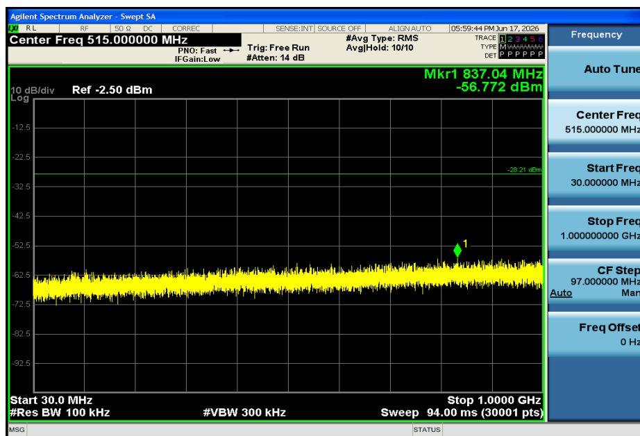
11B-Ant1-2412-30~1000-PASS
