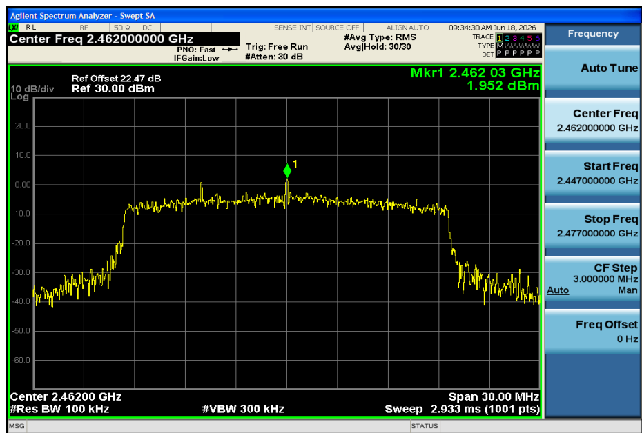
11AX20SISO-Ant1-2462-0~Reference-PASS
