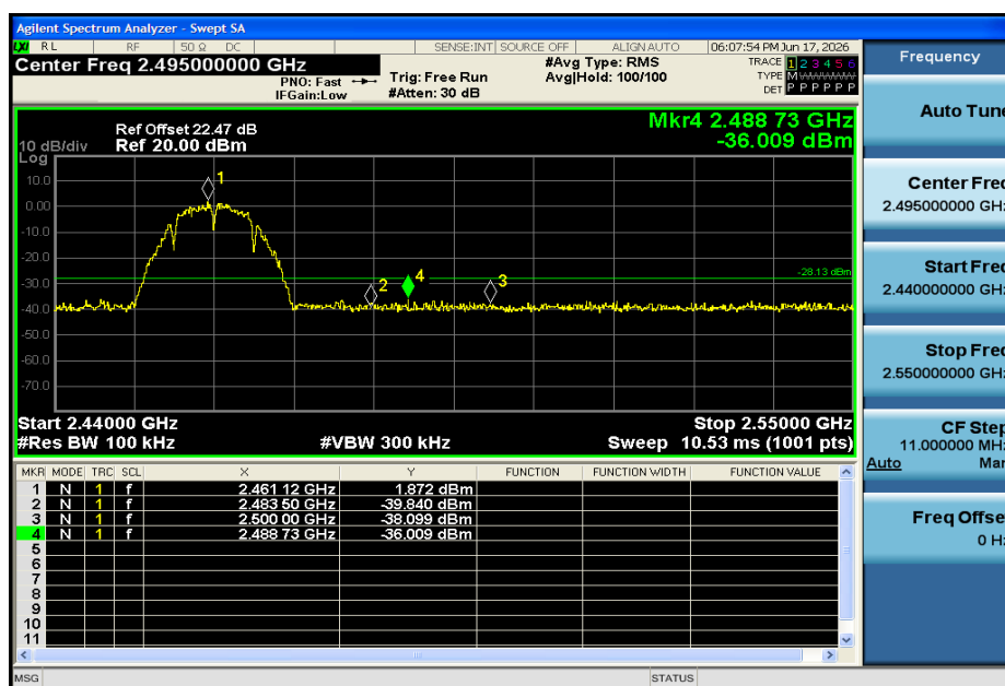
11B-Ant1-2462-PASS
