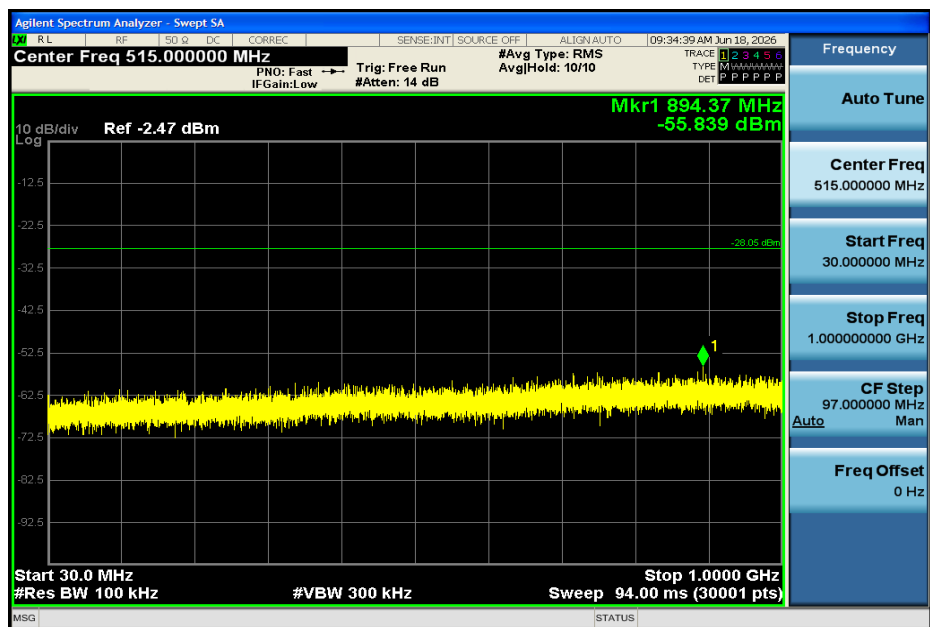
11AX20SISO-Ant1-2462-30~1000-PASS
