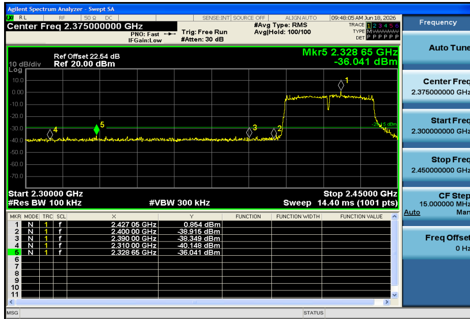
11N40SISO-Ant1-2422-PASS
