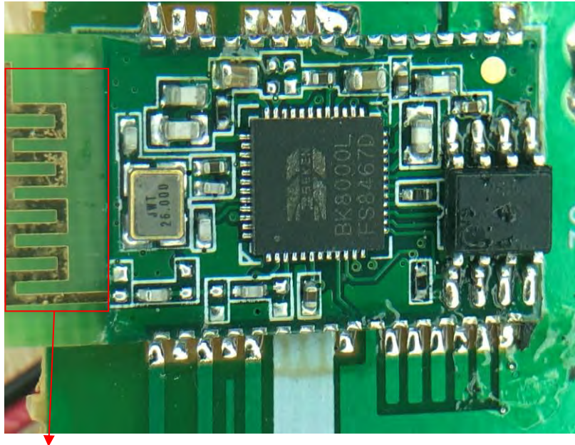
RF Antenna
