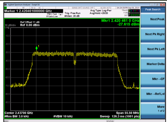
Channel 06 (2437MHz)
