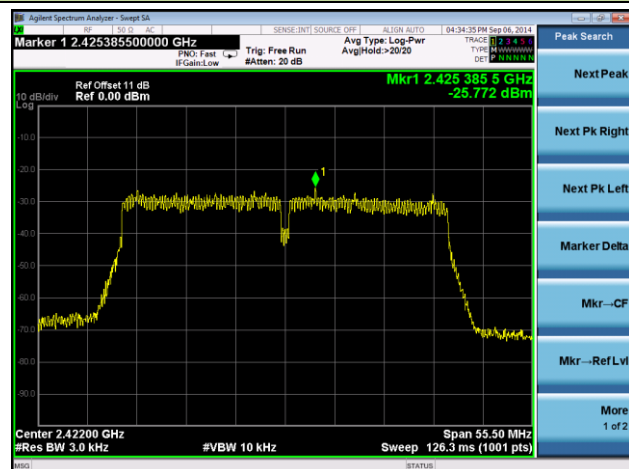
Channel 03 (2422MHz)
