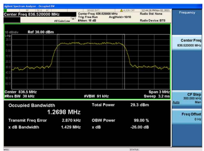
CDMA BC0 (1xRTT), CH384, 836.52MHz
