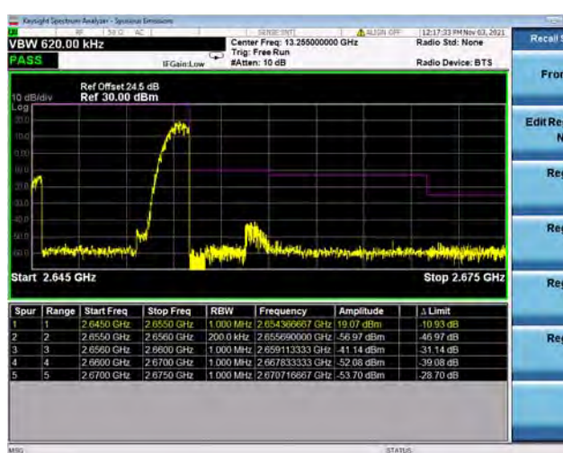
Band41 / 10MHz / High CH / QPSK / 1 RB
