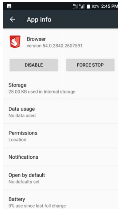
Figure 7-27 Applications
