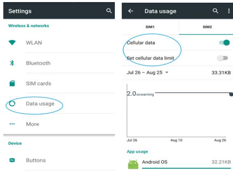
Figure 7-9 Data usage
