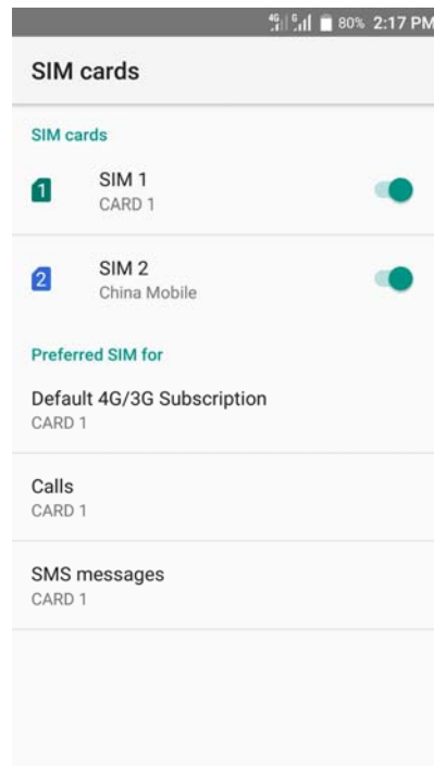
Figure 7-8 SIM cards
