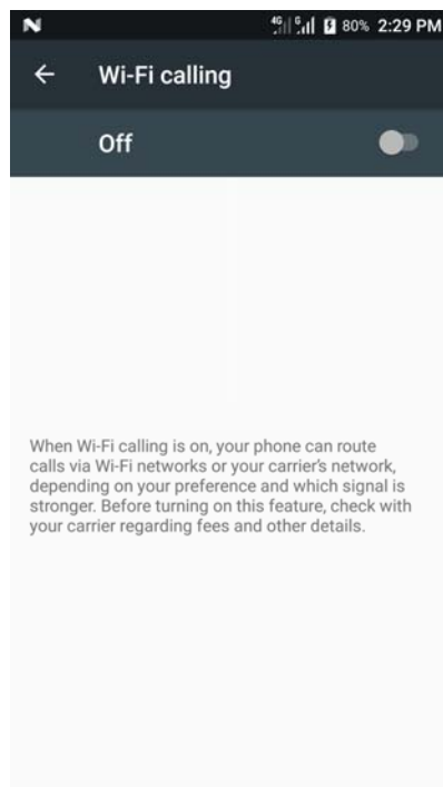
Fig 7-12 WIFI calling
