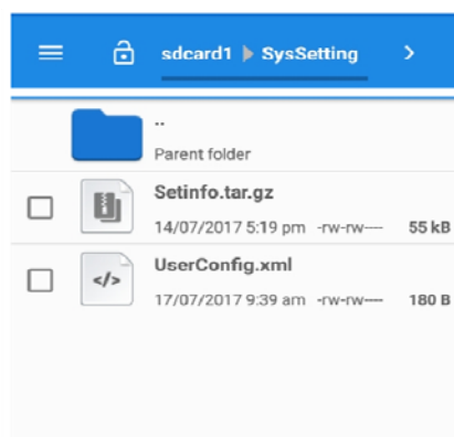
Figure 8-35 User profile
