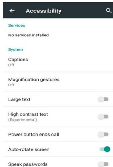
Figure 7-37 Accessibility
