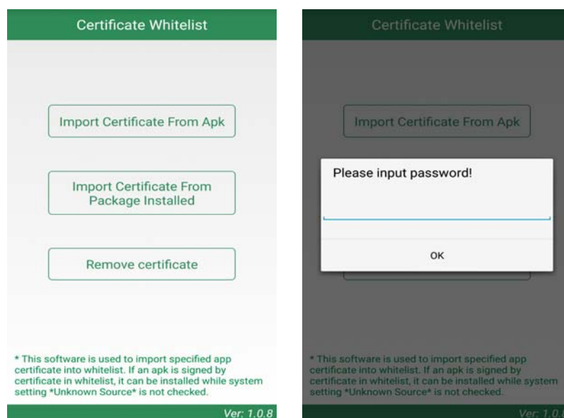
Figure 8-38 Certificate Whitelist
