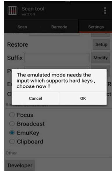
Figure 8-6 EmuKey settings
