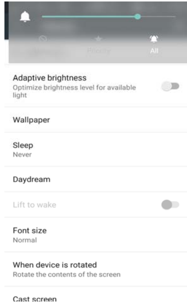
Figure 7-20 Display
