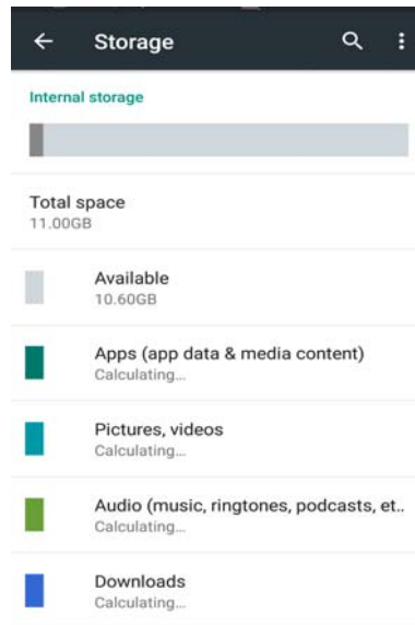
Figure 7-28 Storage
