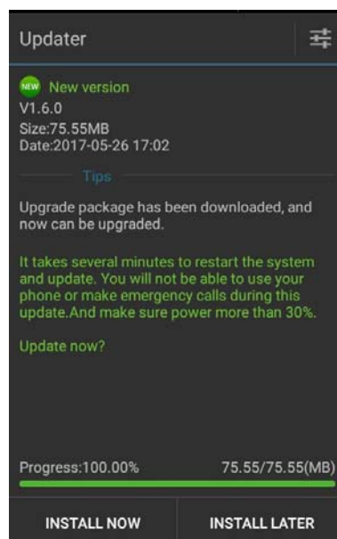
Figure 8-11 Update now
