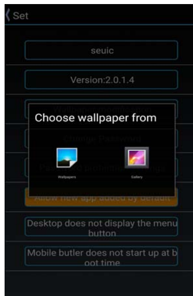
Figure 8-22 Wallpaper modification
