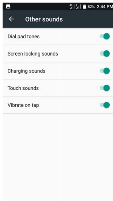
Figure 7-26 Sound
