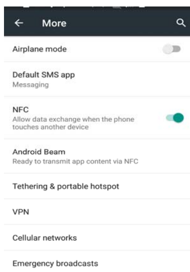
Figure 7-11 NFC feature
