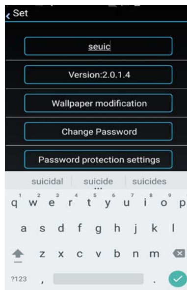
Figure 8-21 Change name
