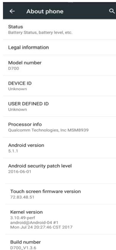
Figure 7-39 About phone
