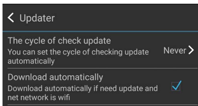
Figure 8-13Settings
