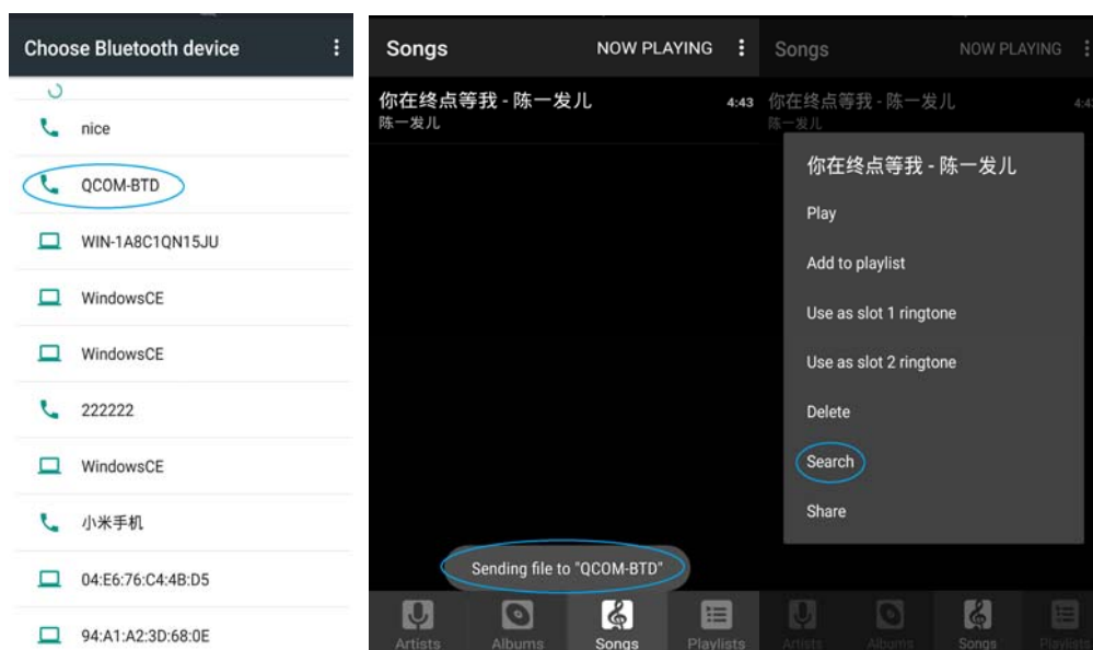
Figure 7-5 Bluetooth transmission
