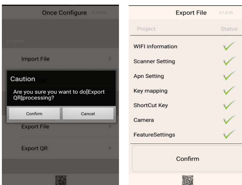
Figure 8-33 Export QR
