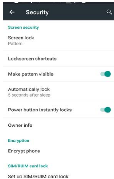
Figure 7-32 Security
