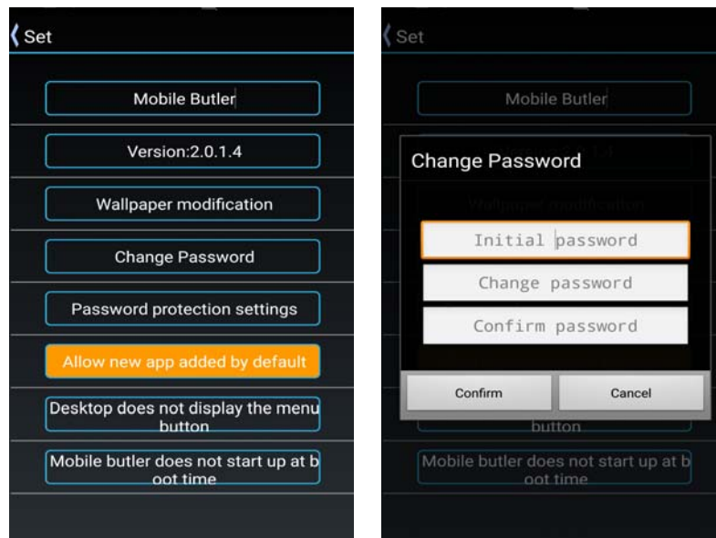
Figure 8-20 Change password
