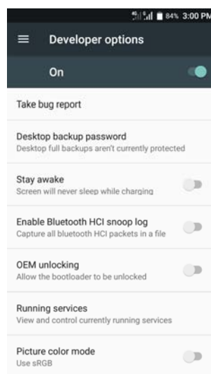
Figure 7-38 Developer options
