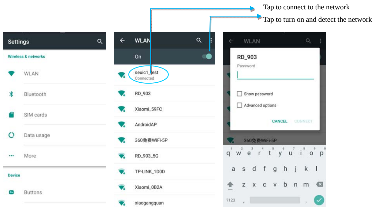
Figure 7-1 Wi-Fi menu
