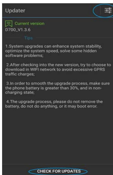
Figure 8-9 System update
