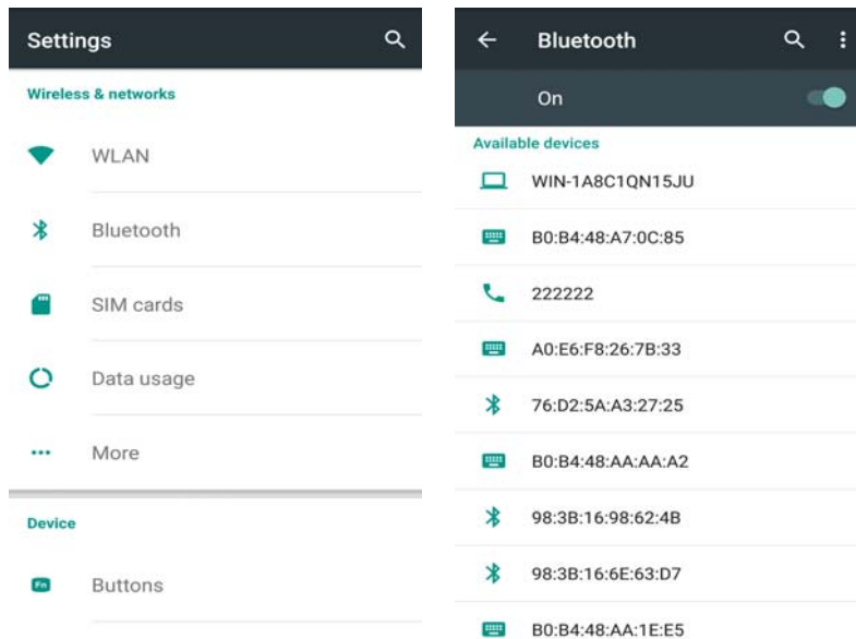
Figure 7-3 Bluetooth menu
