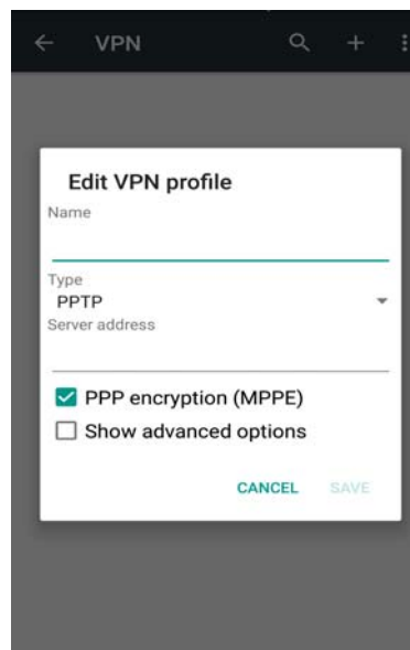
Figure 7-15 VPN Setting
