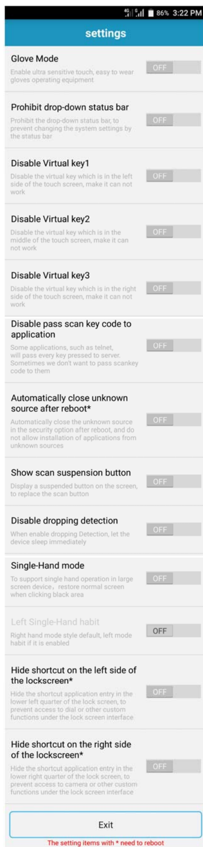
Figure 8-37 Features setup
