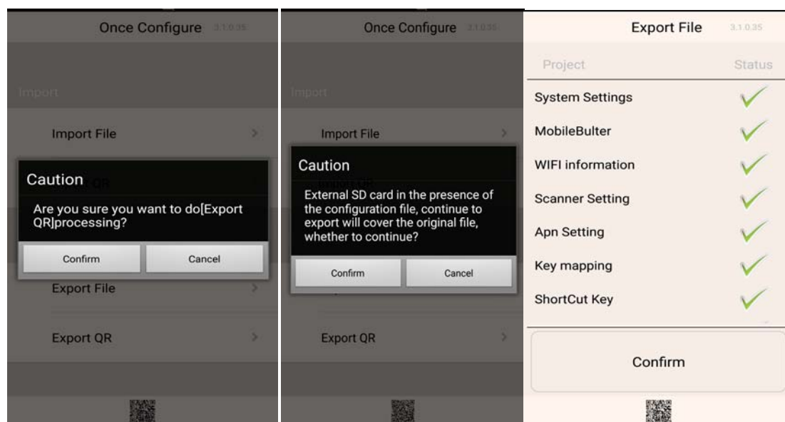
Figure 8-31 Export file
