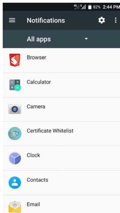
Figure 7-25 Notification
