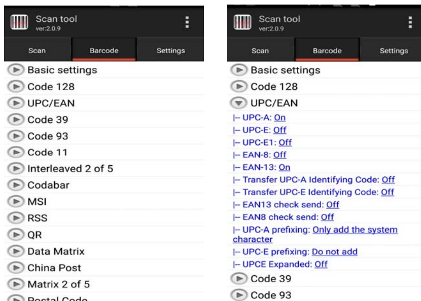
Figure 8-2 Barcode
