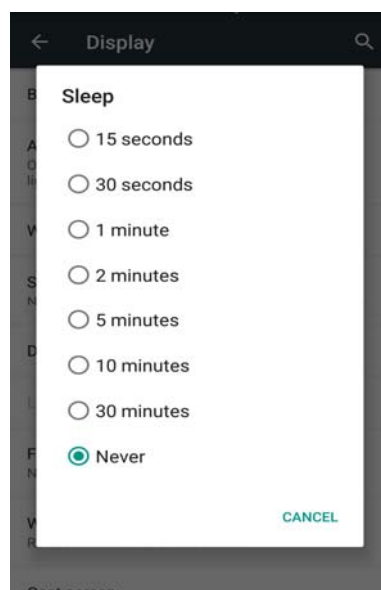
Figure 7-23 Sleep mode
