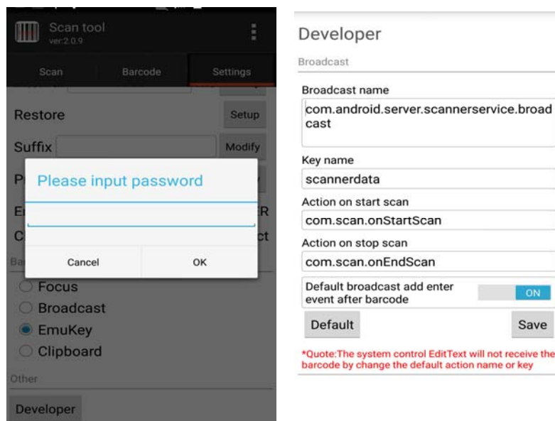
Figure 8-7 Developer
