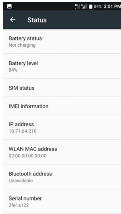
Figure 7-40 Status
