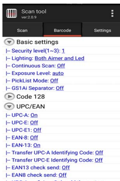
Figure 8-3 Basic settings
