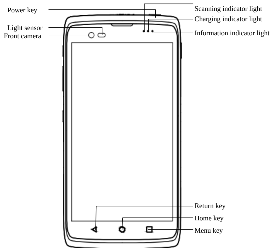
Figure 2-1 Front view
