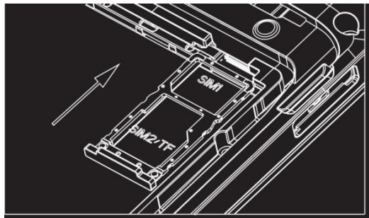
Figure 4-1 Placement of SIM Card
